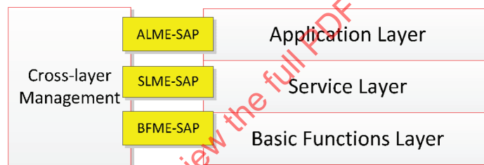
Figure 6 — Service access point provided by I/F CLM / (AL-SL-BFL)
