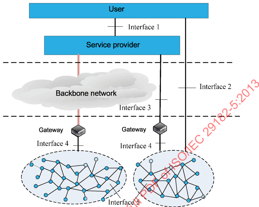
Figure 7 — Interfaces between entities enabling SN services and applications
