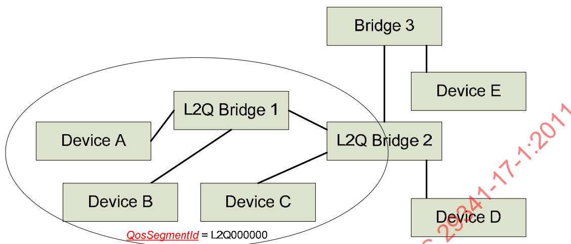
Figure 11 — A network with Ethernet Layer-2-QoS bridges, L2Q-end point devices and legacy Ethernet bridges and legacy Ethernet devices
