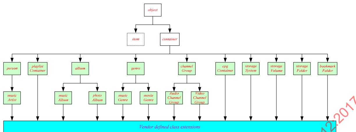
Figure C.2 — Class hierarchy for the container base class
