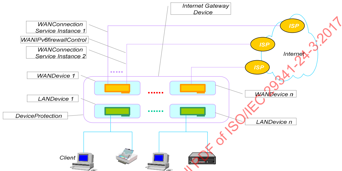
Figure 1 — InternetGatewayDevice with LAN and WAN Interfaces
