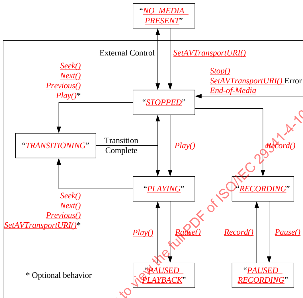
Figure 1: TransportState Transitions - INFORMATIVE
