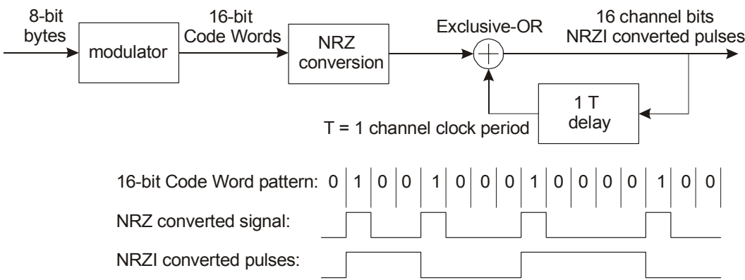
Figure 16 — NRZI conversion
