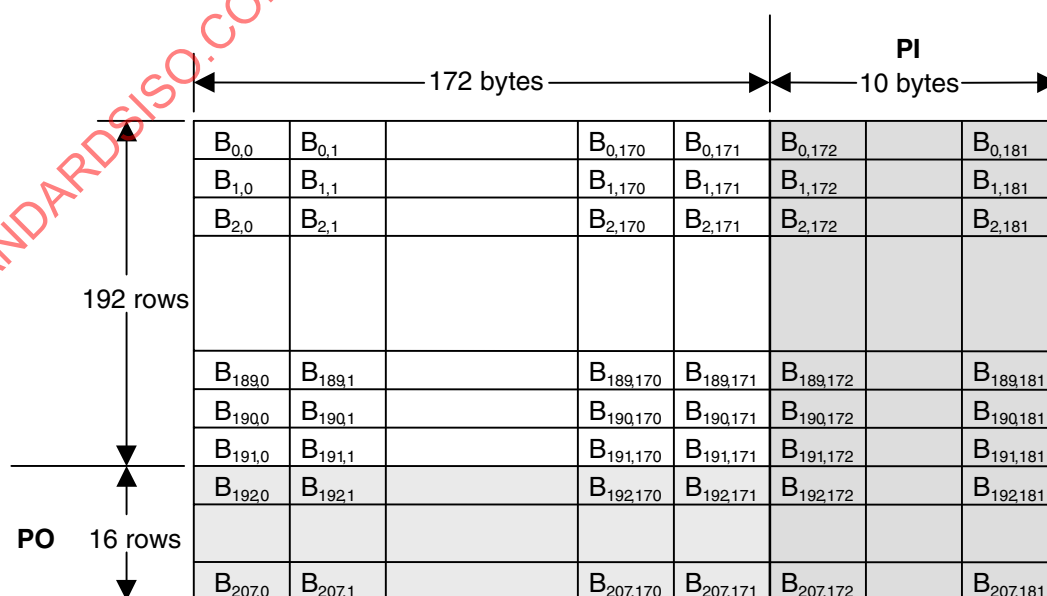
Figure 14 — ECC Block
