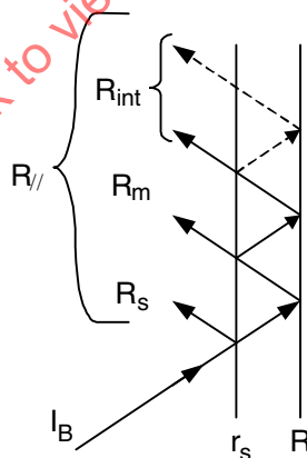
Figure C.1 — Reflectivity calibration
