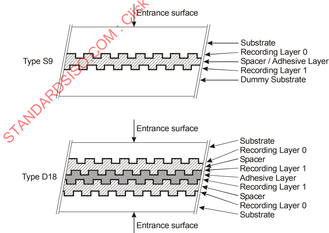
Figure 1 — Types of +RW DL disk
