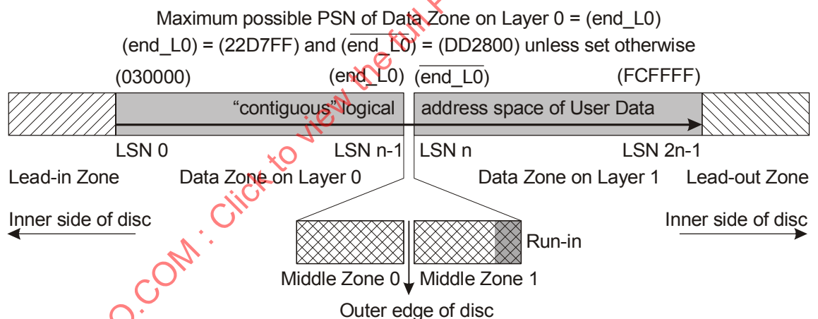
Figure 24 — Contiguity of Data Zones
