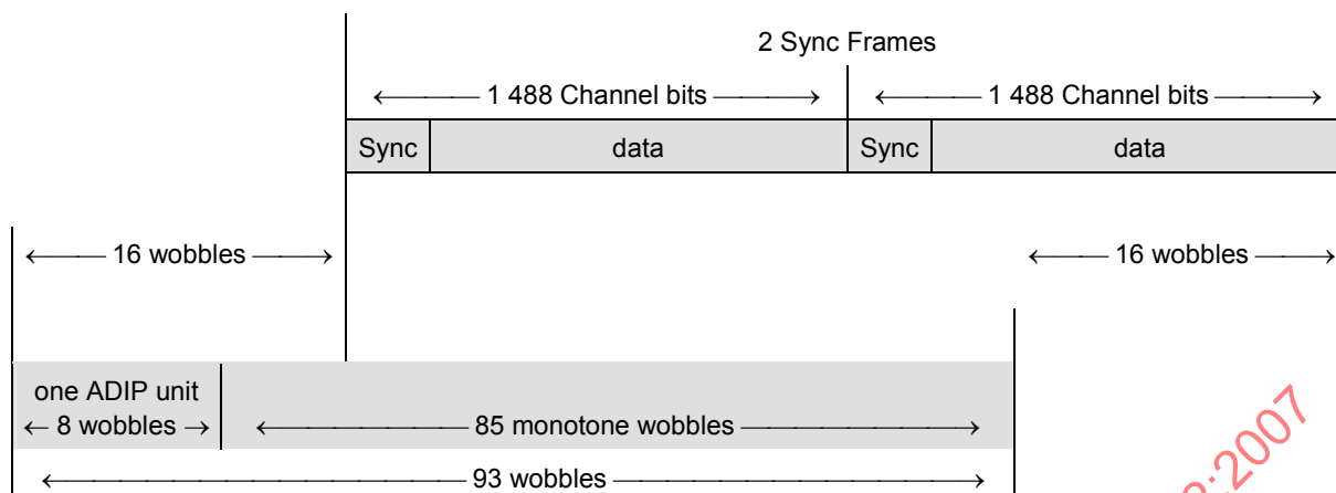
Figure 19 — General ADIP structure
