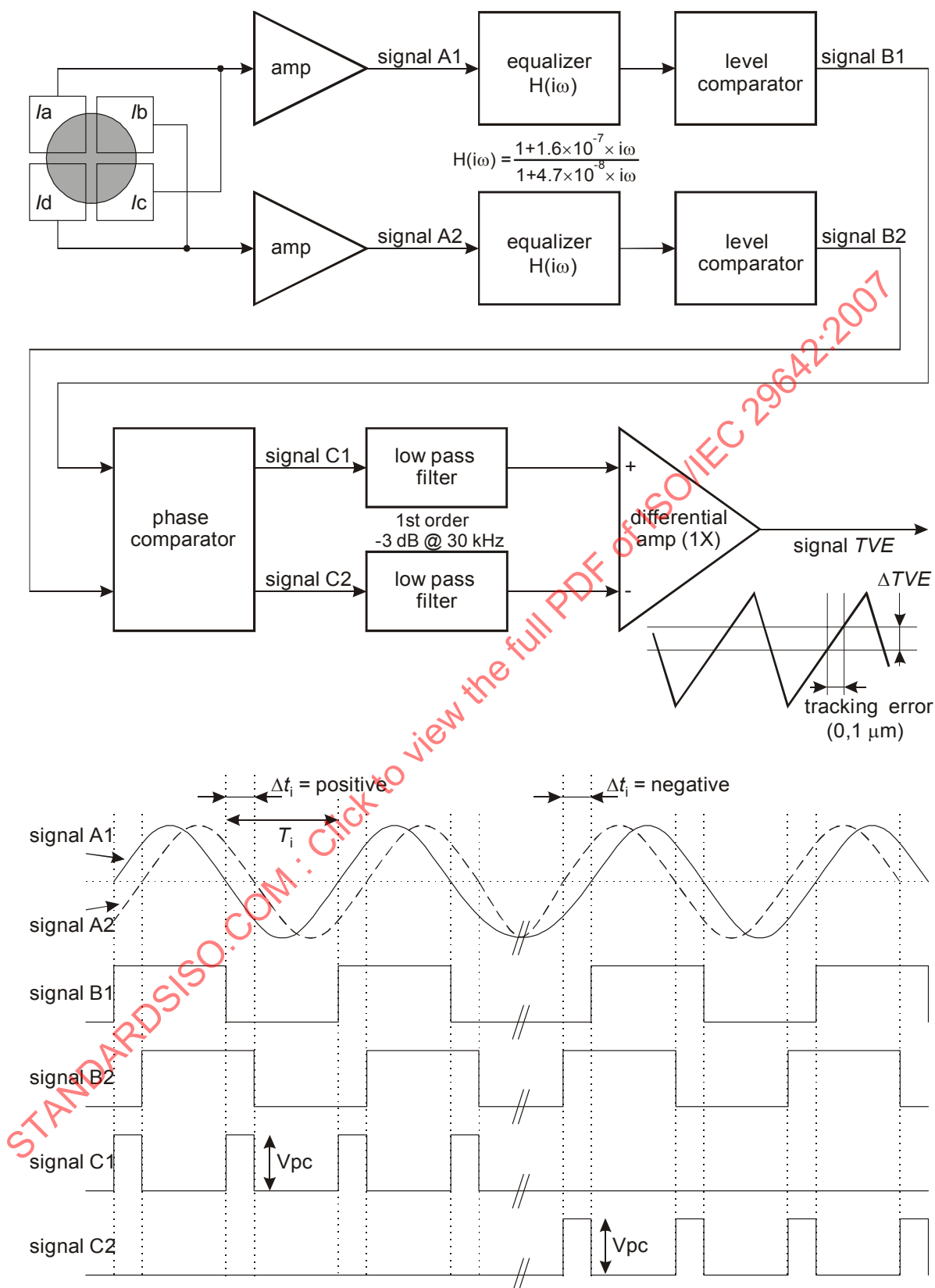
Figure F.1 — Circuit for tracking error measurements
