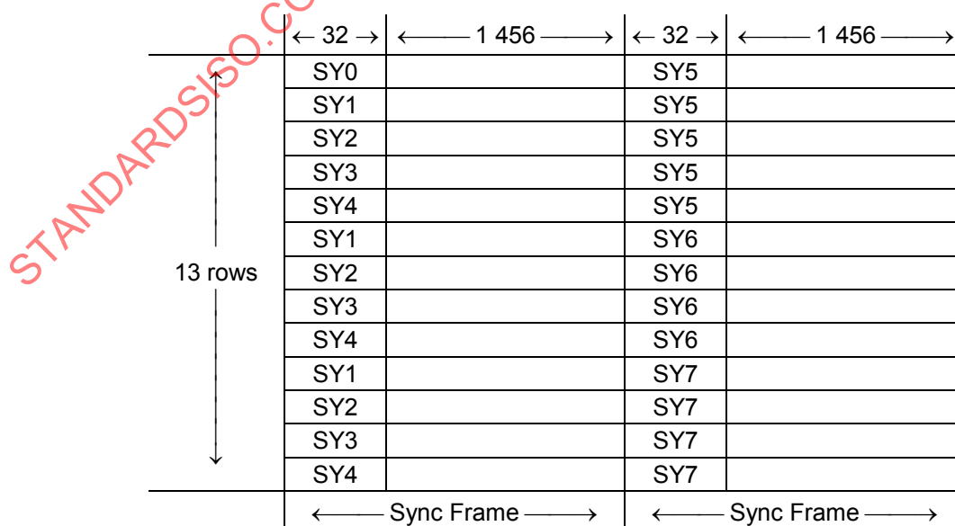
Figure 17 — Physical Sector
