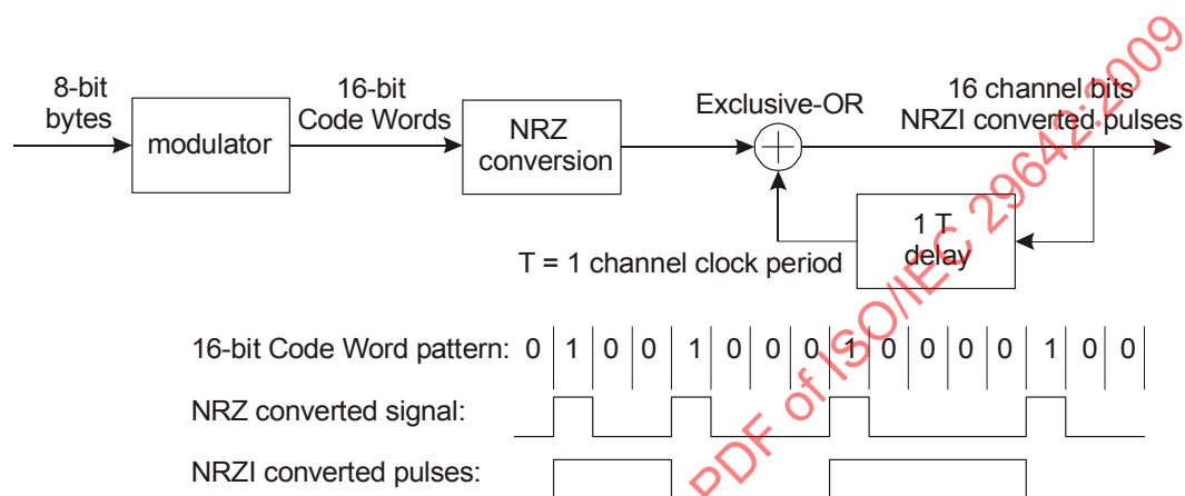
Figure 16 — NRZI conversion
