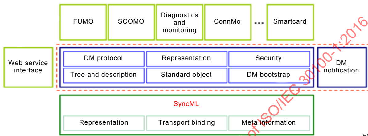
Figure B.4 – OMA DM protocol stacks
