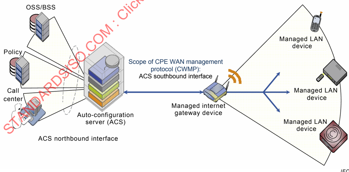
Figure B.1 – TR-069 positioned as an end-to-end architecture
