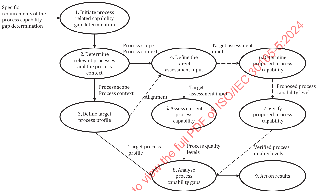
Figure 5 — Steps of process capability gap determination
