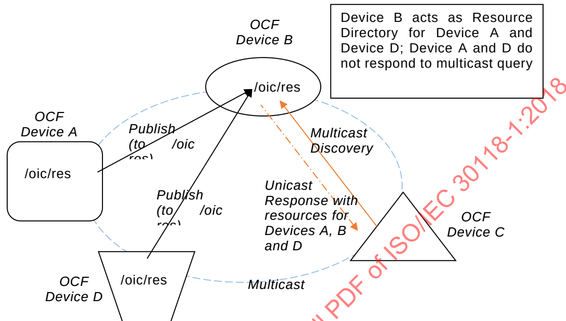
Figure 26. Indirect discovery of resource by resource directory
