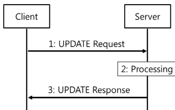
Figure 18. UPDATE operation
