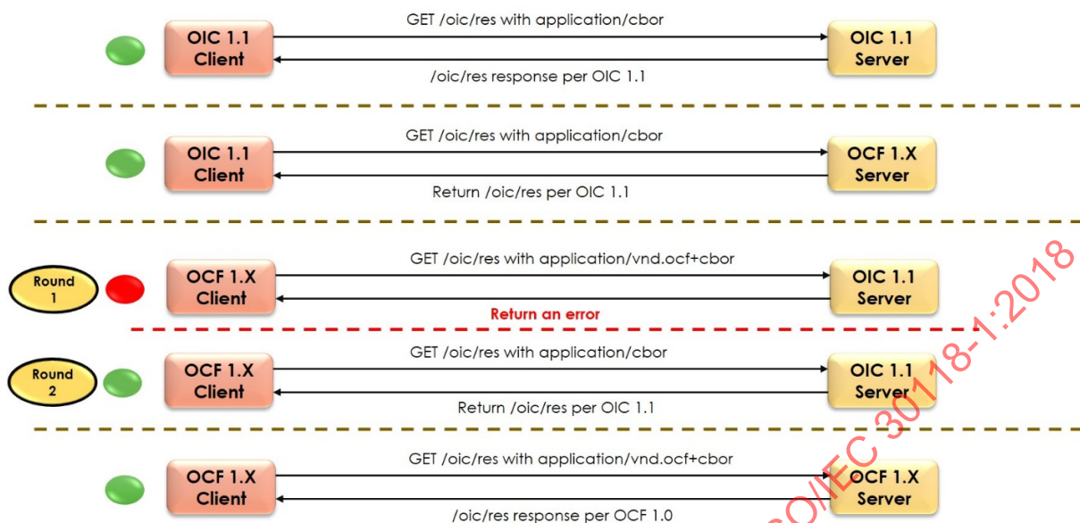
Figure 38 Content-Format Policy
