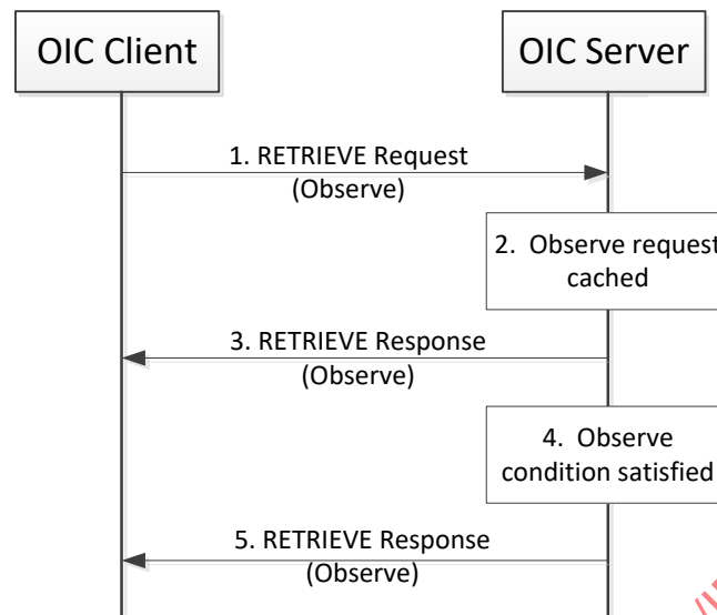
Figure 32. Observe Mechanism
