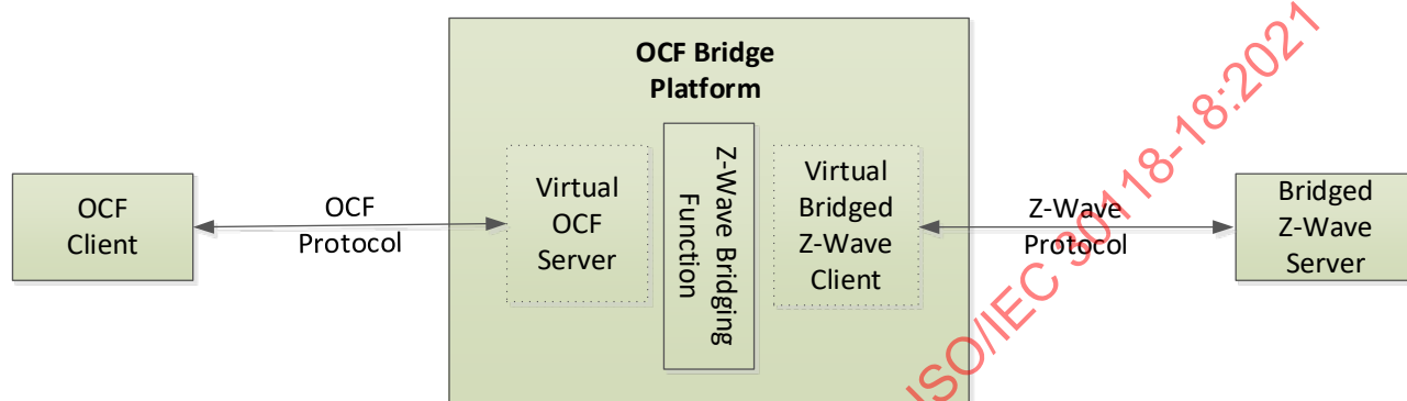
Figure 1 – OCF Z-Wave Bridge Platform and Components
