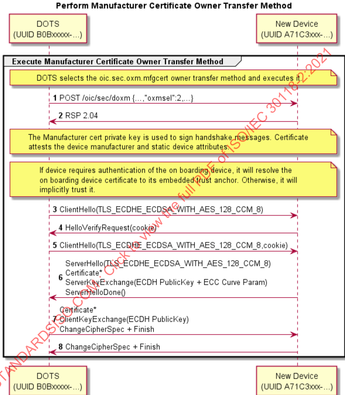
Figure 12 – Manufacturer Certificate Based OTM Sequence
