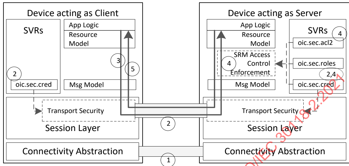
Figure 2 – OCF layers
