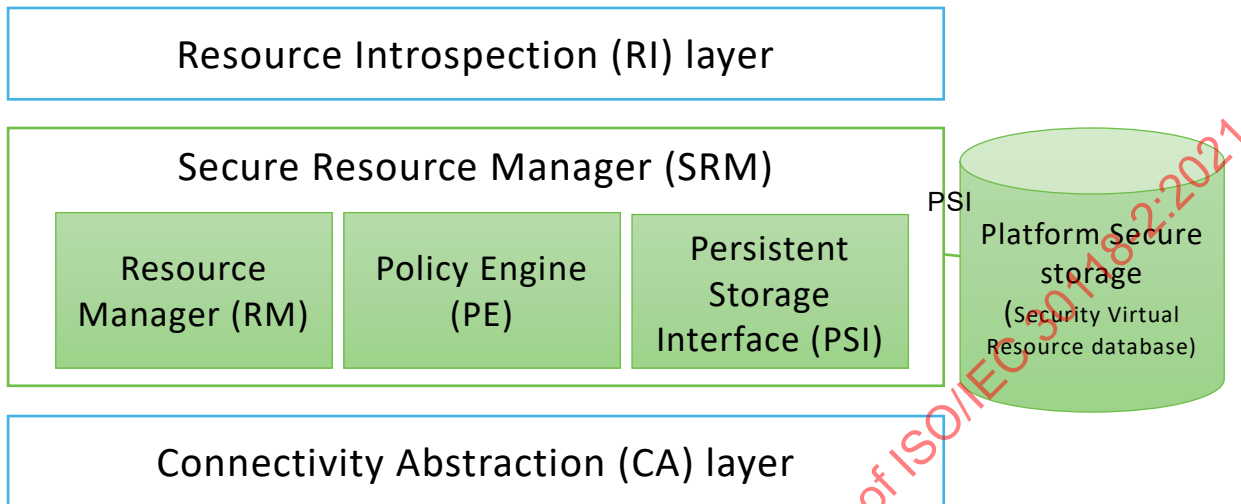
Figure 7 – OCF's SRM architecture
