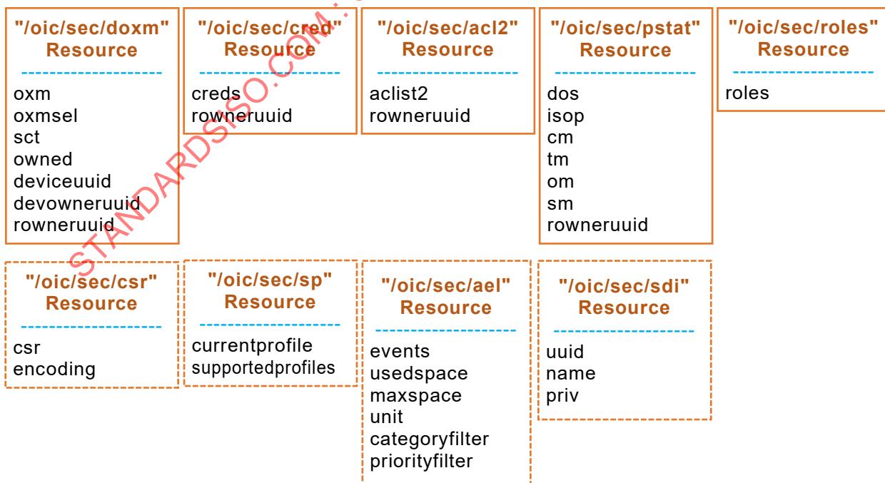
Figure 19 – OCF Security Resources
