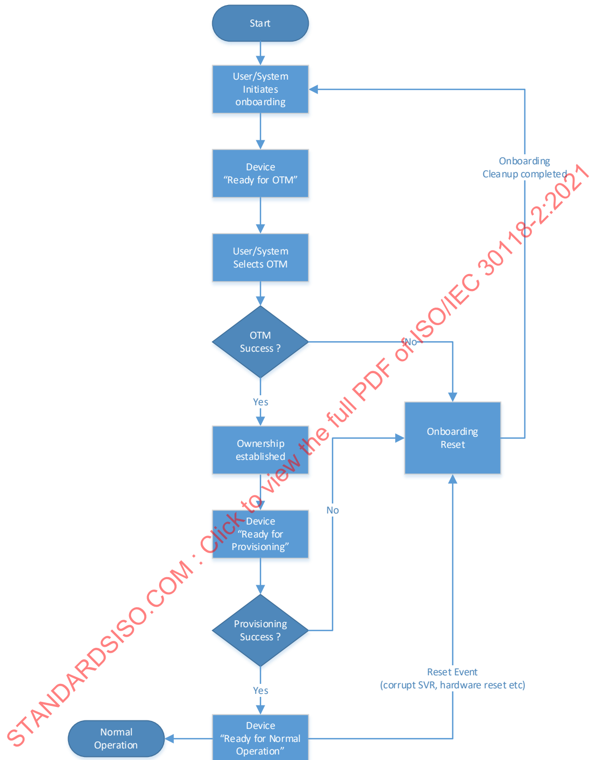
Figure 6 – OCF onboarding process
