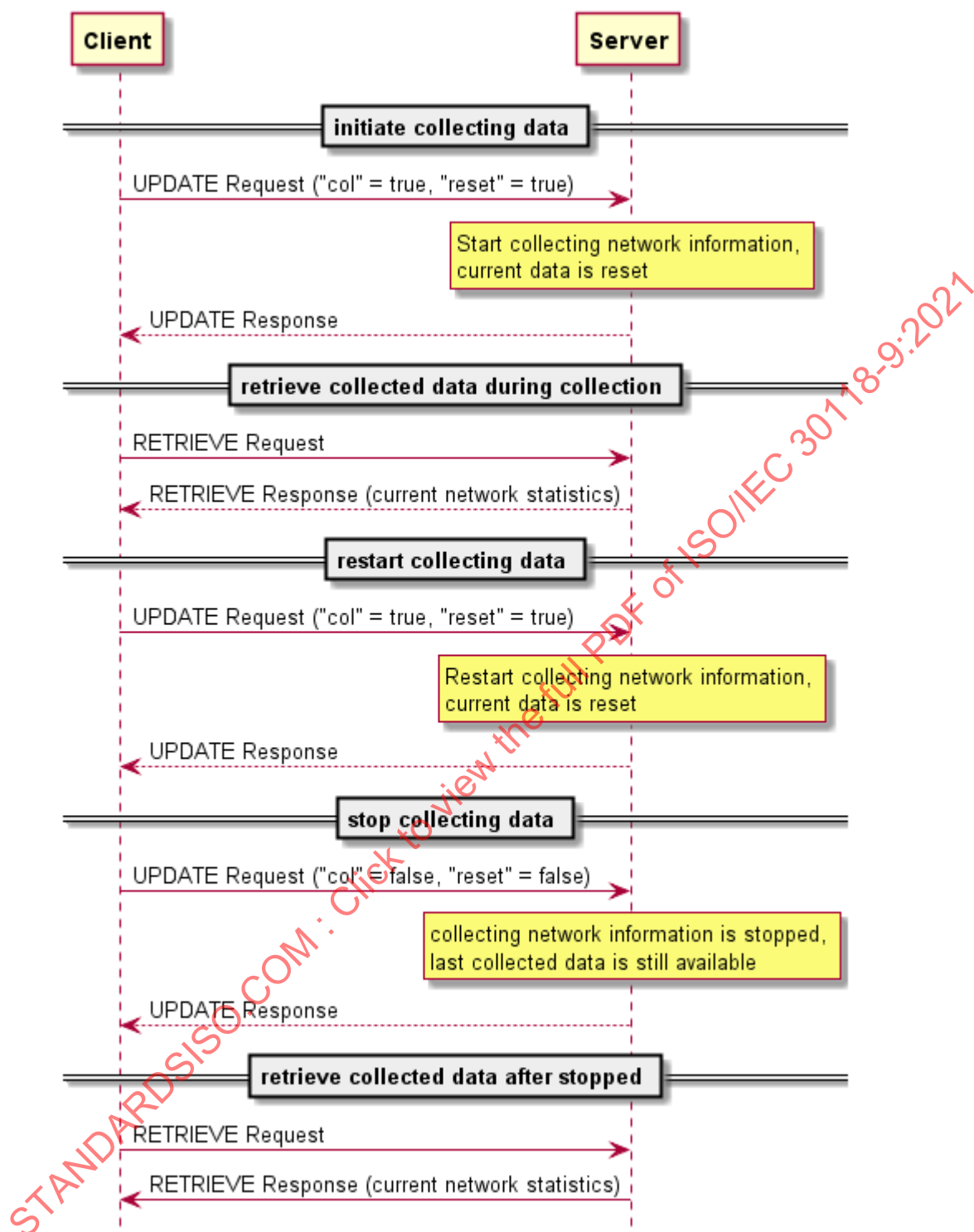
Figure 1 – Interactions with the network monitoring Resource
