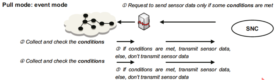
Figure 6 — Sensor data collection: Pull mode-event mode
