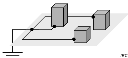
Figure 10 a – Star local protective bonding network
