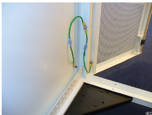
Figure 4 – Example of a bond connection from a cabinet to the cabinet door
