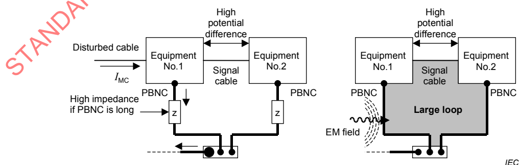
Figure 11 – Example of high common impedance and large loop
