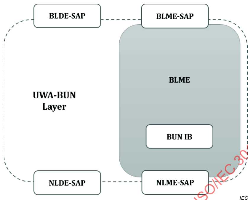
Figure 16 – UWA-Bundle layer reference model
