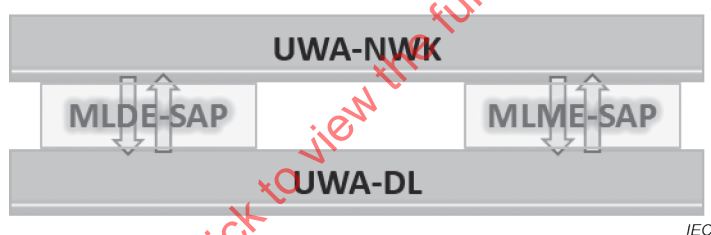
Figure 11 – Service access point provided by the UWA-DL / NWK
