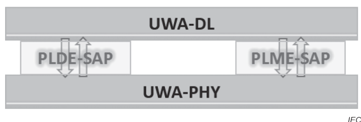
Figure 10 – Service access point provided by the UWA-PHY / DL
