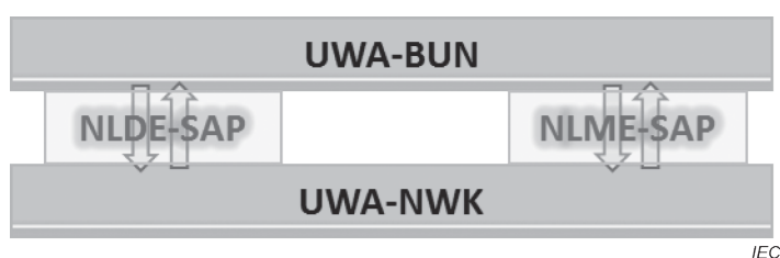
Figure 12 – Service access point provided by the UWA-NWK / BUN
