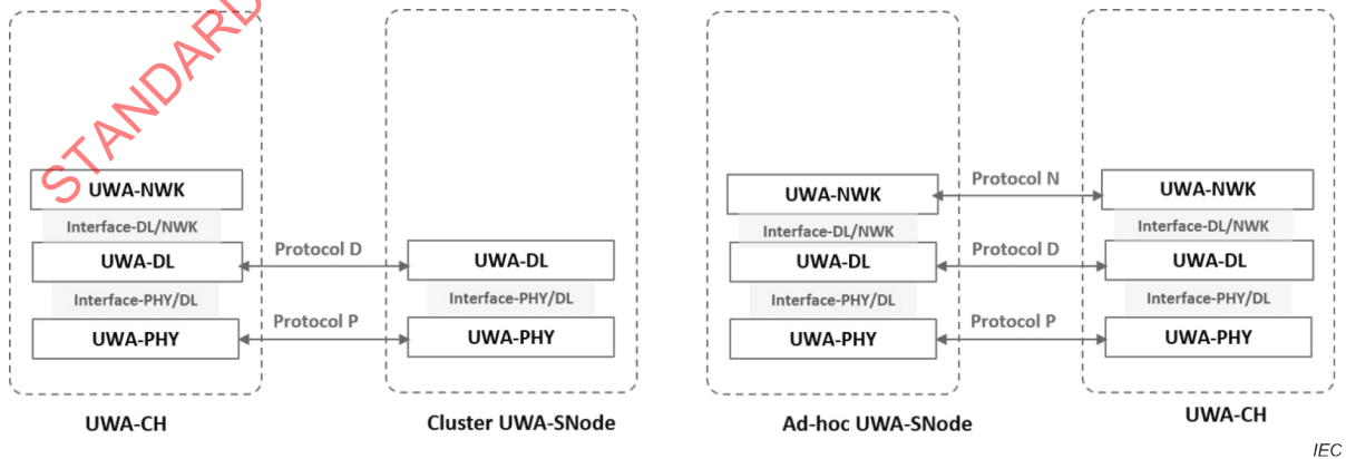
Figure 8 – Information exchange in different layers via interface 4
