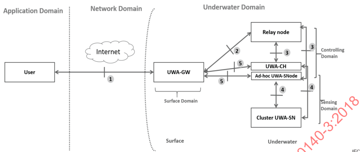
Figure 4 – Functional view of interfaces between the physical entities
