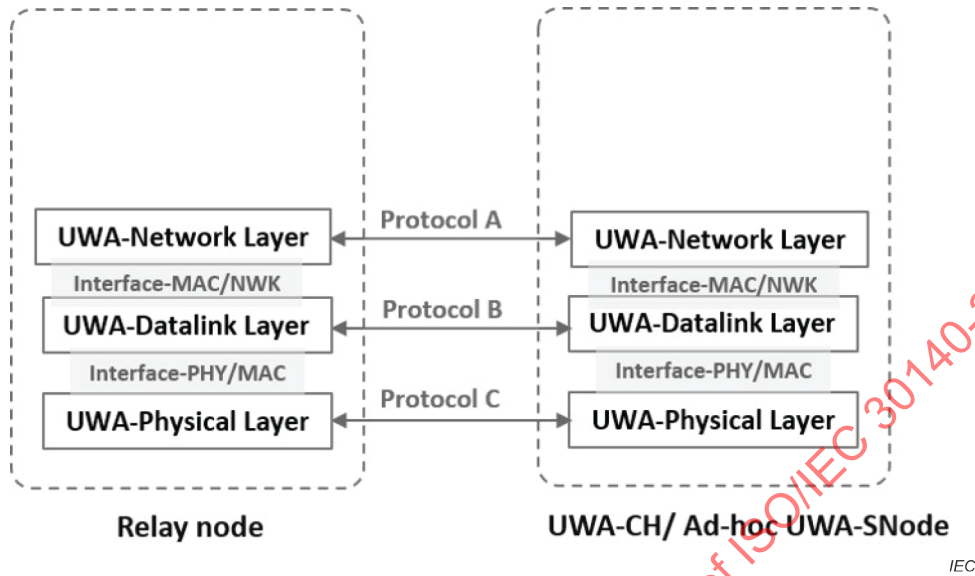
Figure 7 – Information exchange in different layers via interface 3
