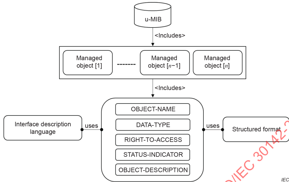
Figure 4 – General format of u-MIB
