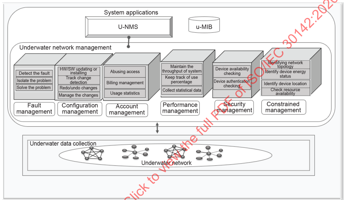
Figure 2 – Functions of the U-NMS
