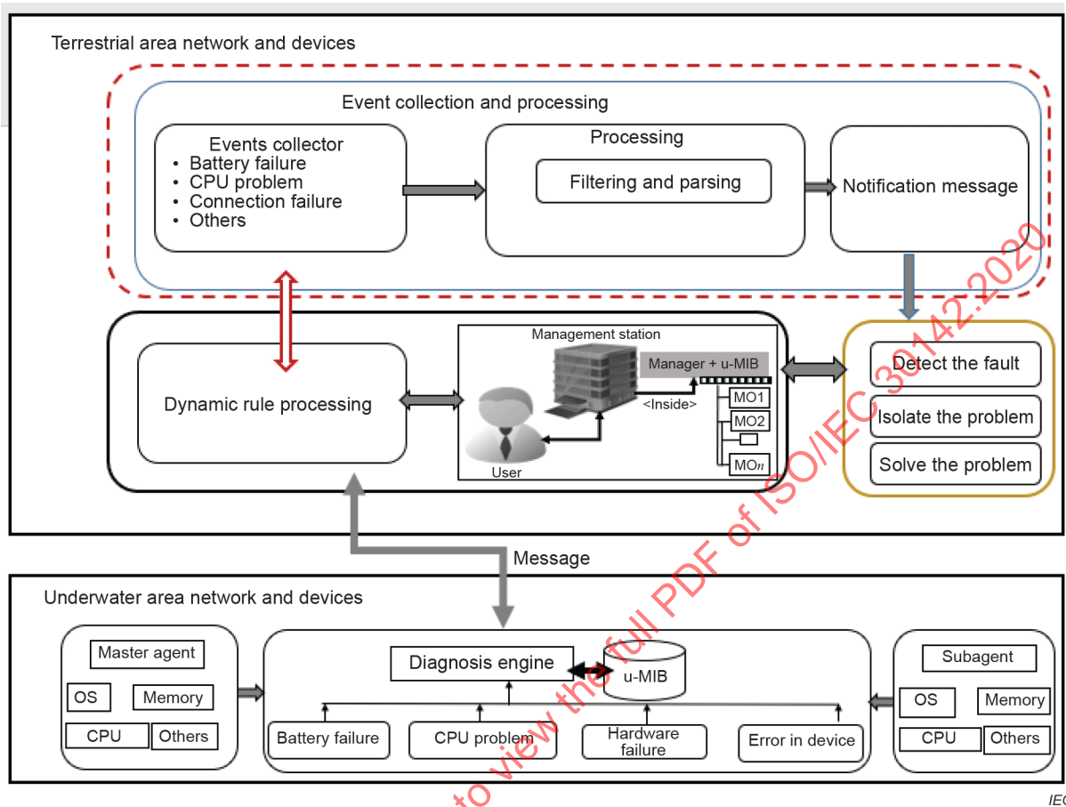
Figure 3 – Fault management in the U-NMS
