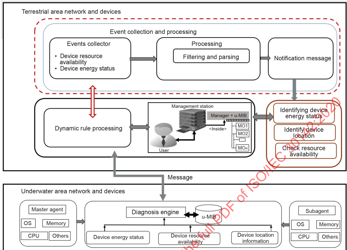
Figure 9 – Constrained device management in U-NMS
