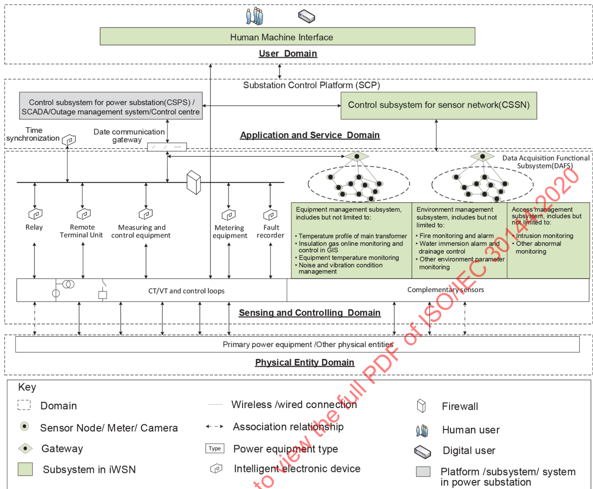
Figure 1 – System overview of the iWSN system supporting electrical power substation
