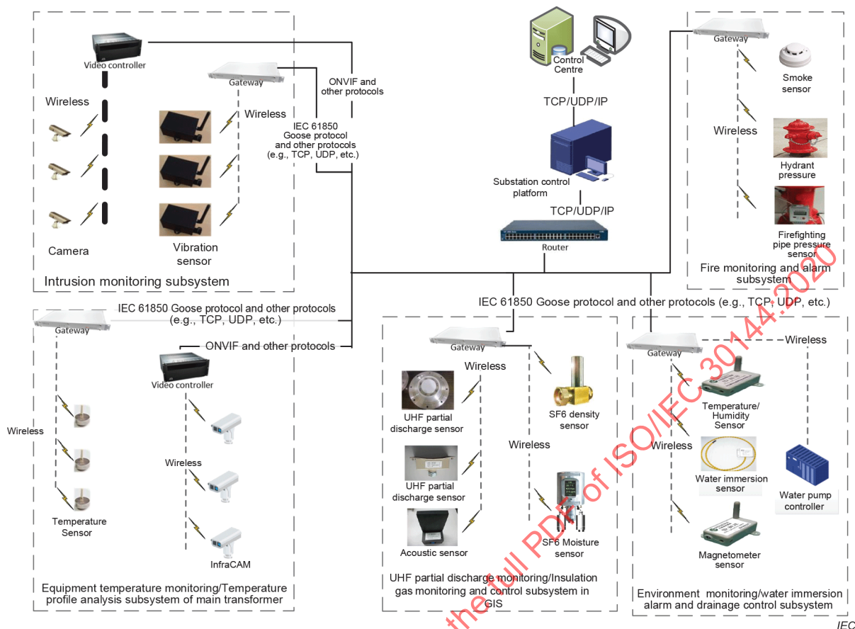
Figure 2 – Communications overview of the iWSN system supporting electrical power substation
