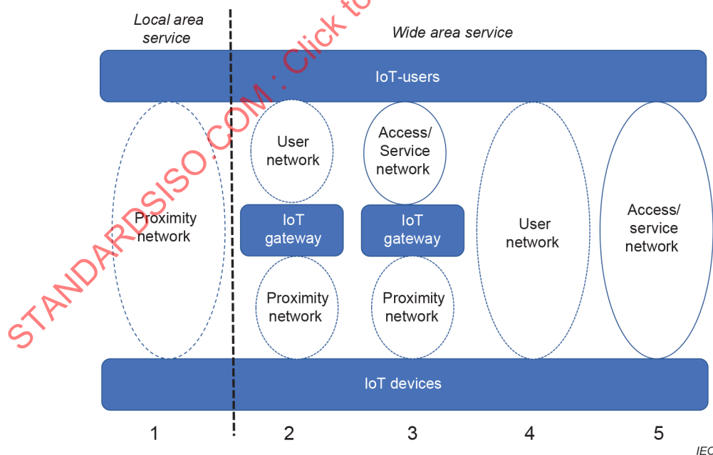
Figure 2 – Service types of the network configurations
