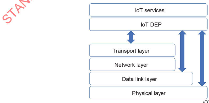
Figure 15 – IoT DEP connections over communication protocols
