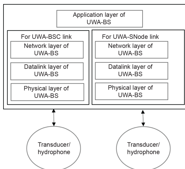
Figure 7 – Overview of UWA-BS communication system
