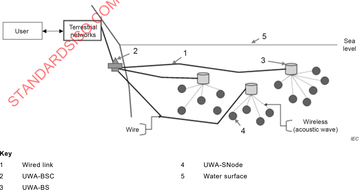
Figure 4 – B-UWAN installation with wired and acoustic communication
