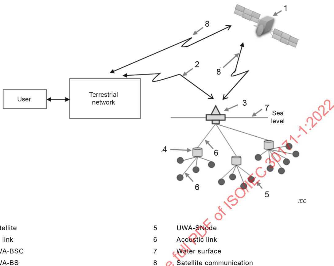
Figure 3 – B-UWAN installation with acoustic communication
