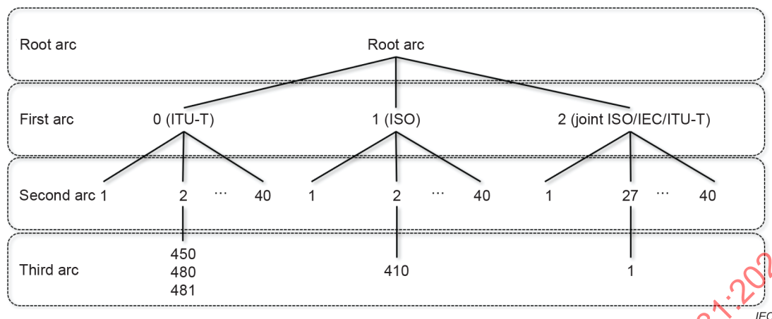
Figure A.1 – International OID tree
