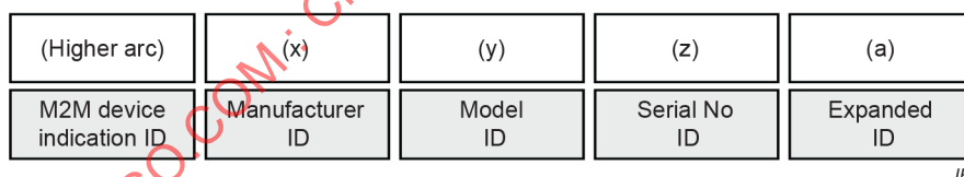
Figure A.2 – oneM2M standard object identifiers
