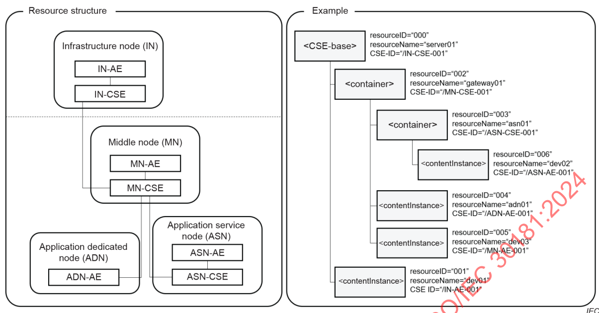
Figure A.3 – oneM2M resource structure
