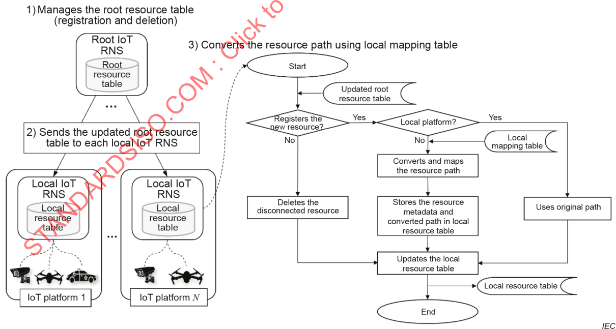
Figure 6 – Discovery service and path conversion in the local IoT RNS
