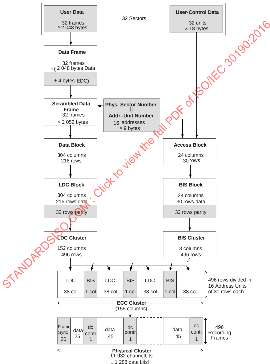
Figure 21 — Schematic representation of encoding process
