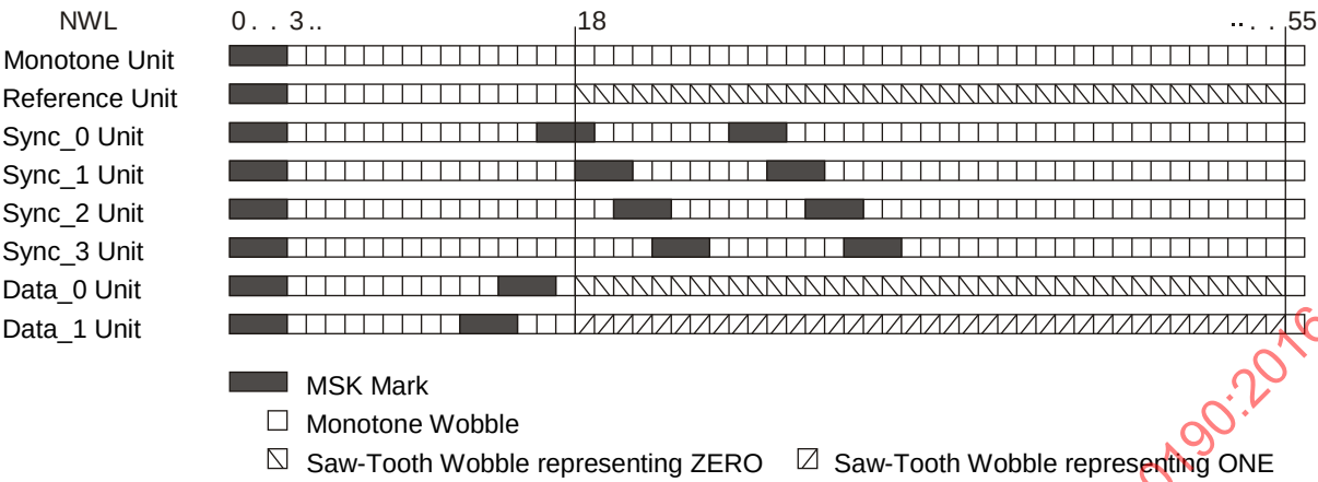
Figure 67 — ADIP-Unit Types
