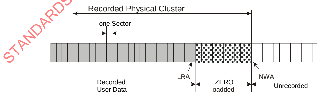
Figure 103 — Example of last RUB with Recorded User Data and padded ZEROS
