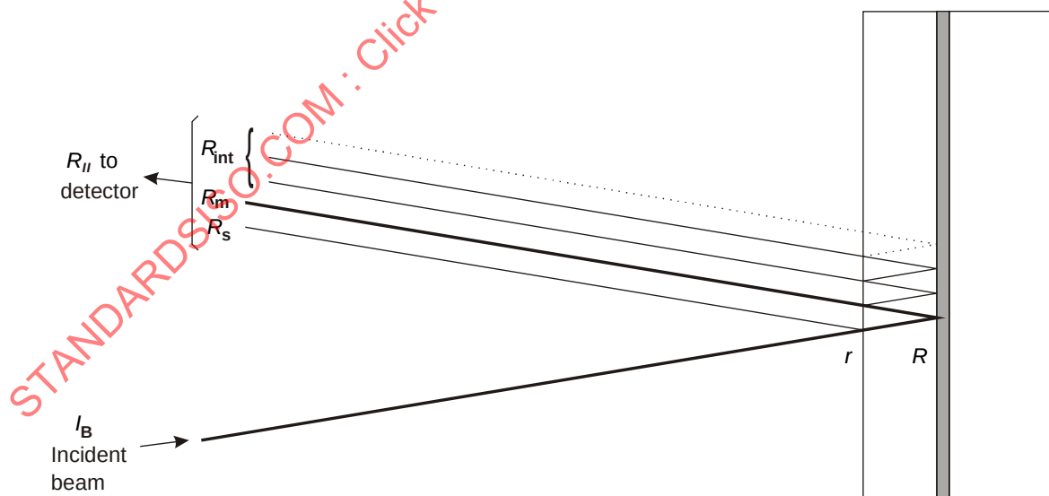
Figure B.1 — Reflectivity calibration
