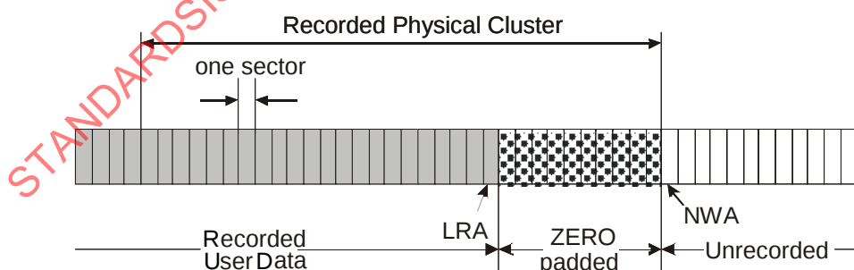
Figure 117 — Example of last RUB with Recorded User Data and padded ZEROs
