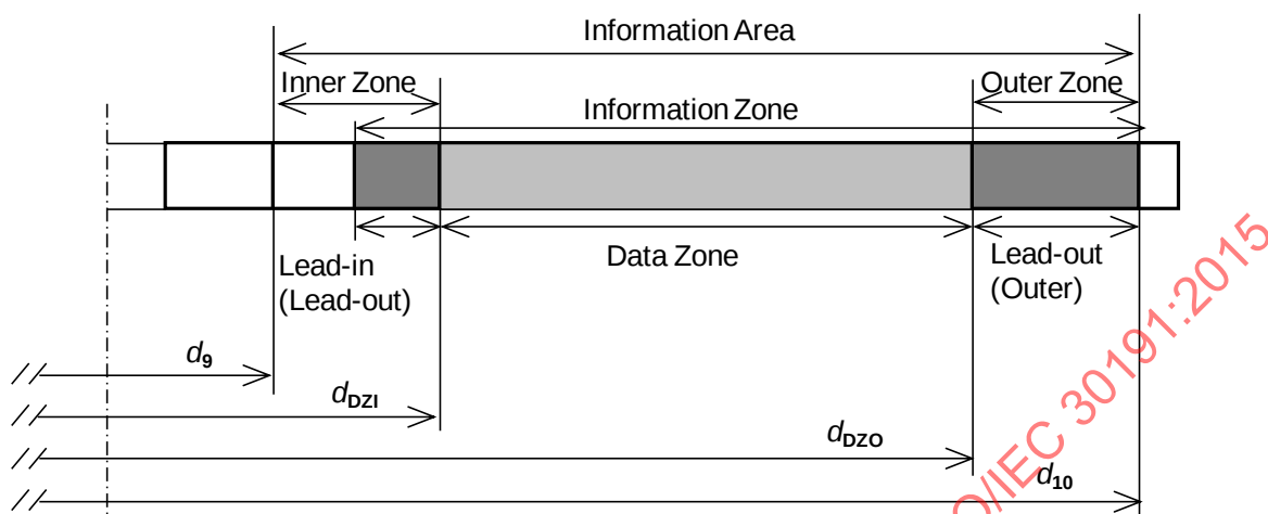
Figure 14 — Division of Information Area
