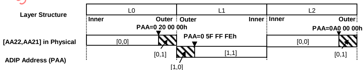
Figure 71 — Combination of AA22 and AA21 for TL disk
