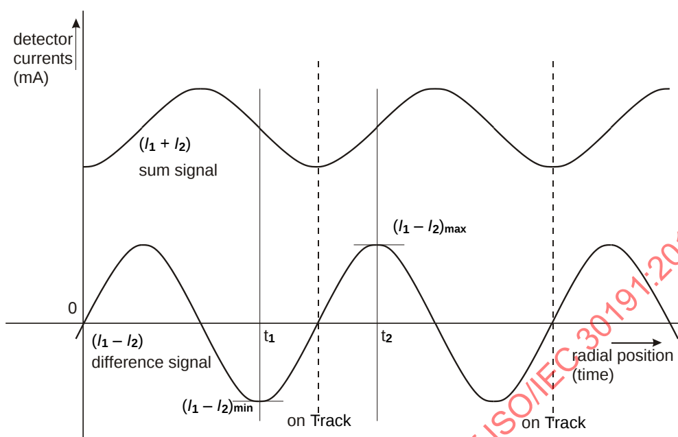
Figure 145 — Definition of Push-Pull signals
