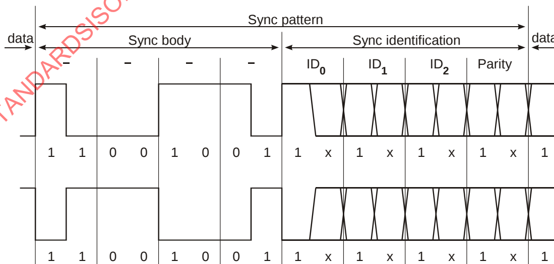
Figure 61 — Biphas Synchronization pattern
