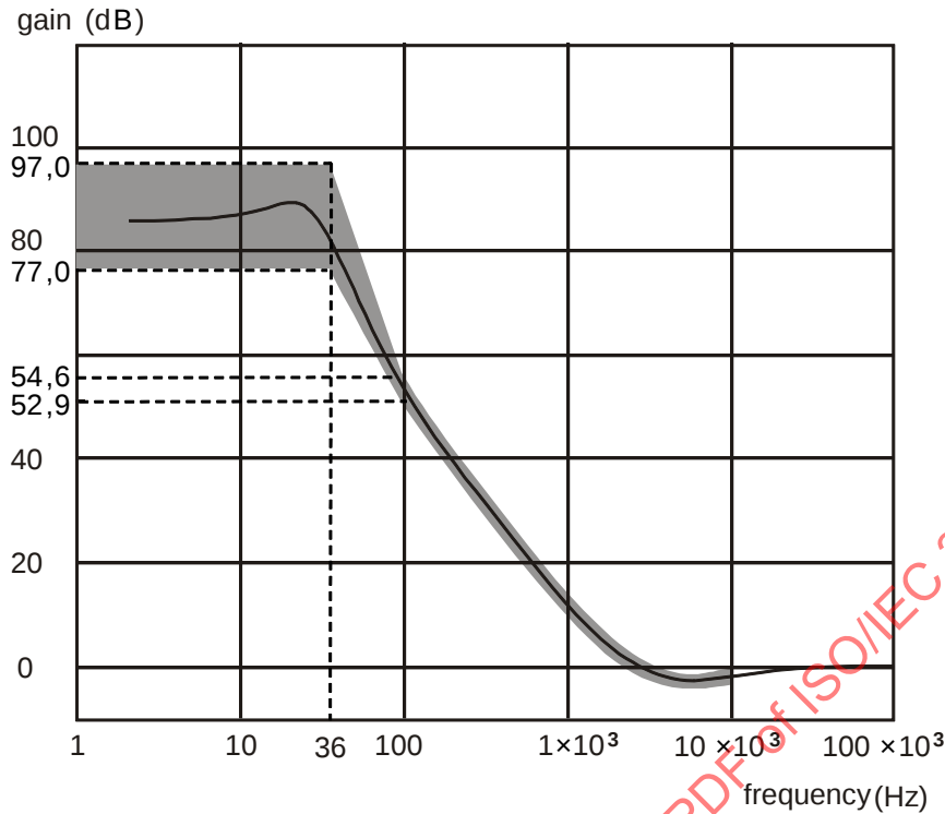
Figure 7 — Servo characteristic for axial tracking at 1x Measurement Velocity
