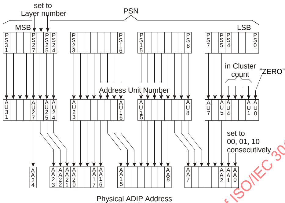
Figure 92 — Physical ADIP Addresses derived from PSN's
