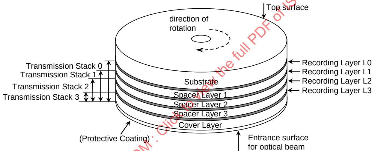
Figure 2 — Outline of Type QL disk
