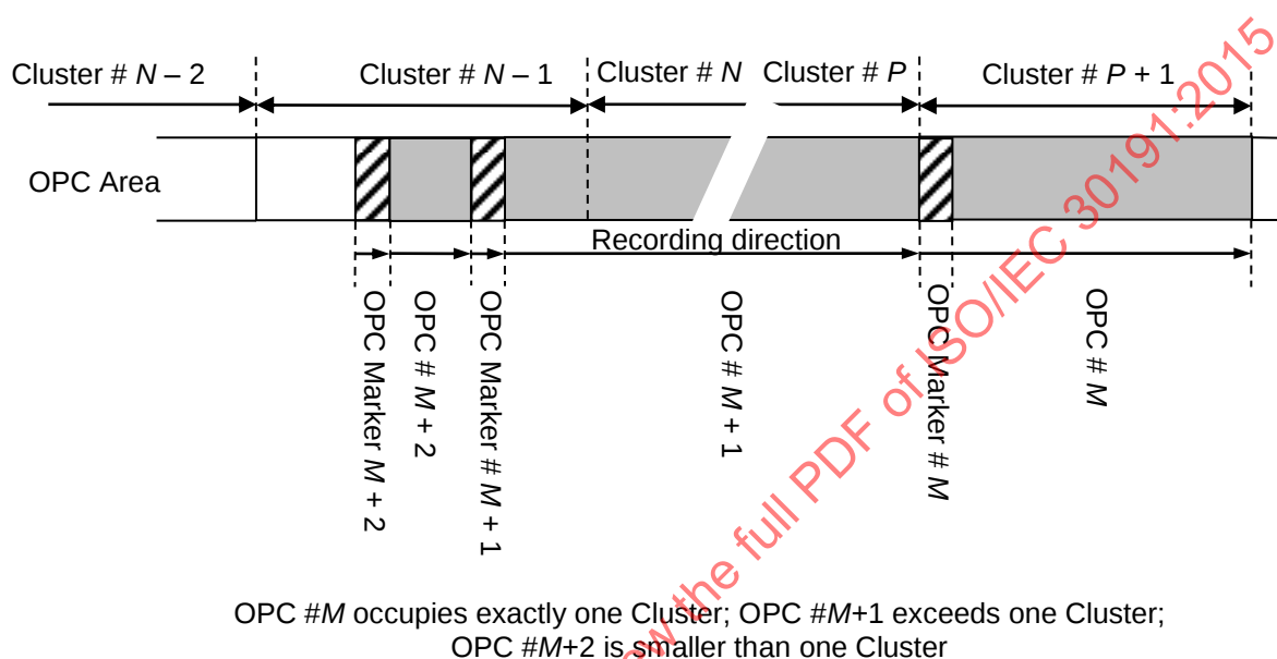
Figure 105 — Example of position of OPC Markers
