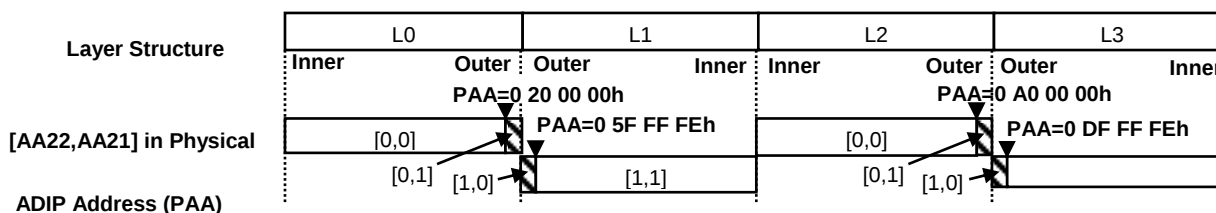
Figure 72 — Combination of AA22 and AA21 for QL disk
