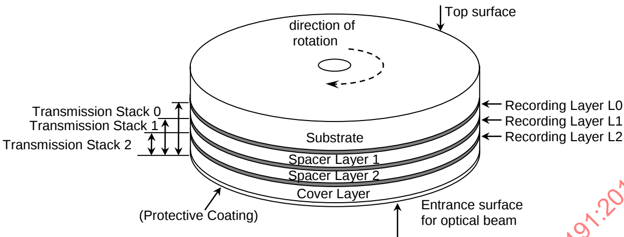
Figure 1 — Outline of Type TL disk
