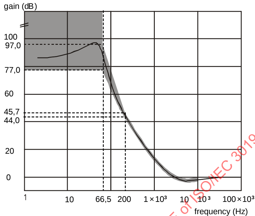
Figure 8 — Servo characteristic for axial tracking at 2x Measurement Velocity
