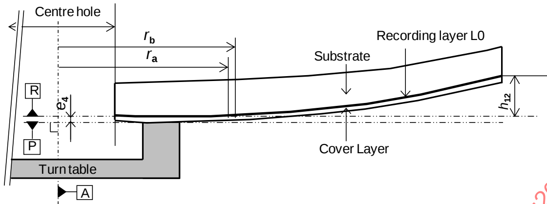
Figure 13 — Details of Disk reference planes P and R and Recording Layer L0
