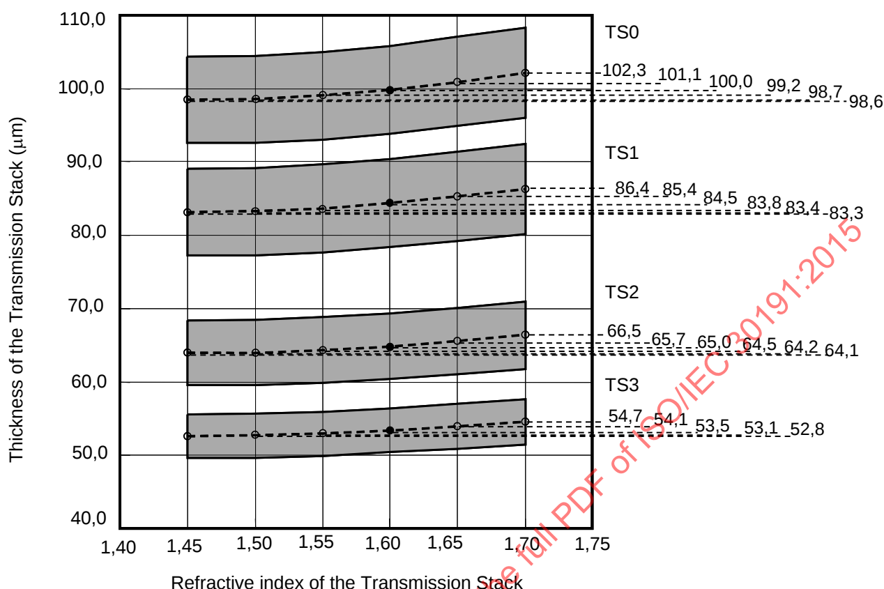
Figure 19 — Thickness of the Transmission Stacks as a function of the refractive index
