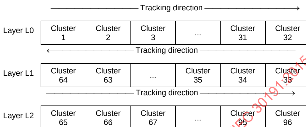
Figure 140 — Clusters of DMAs on TL disk
