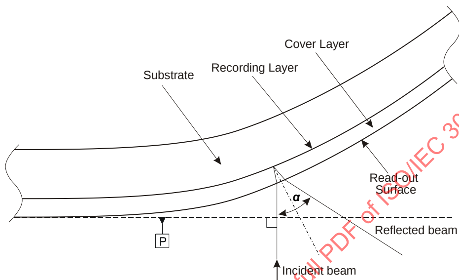
Figure 20 — Definition of angular deviation
