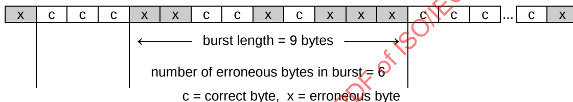
Figure 150 — Example of burst error
