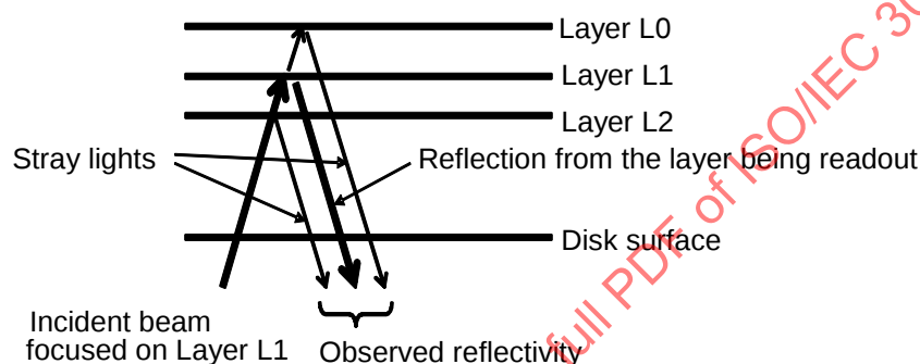
Figure B.2 — Influence of stray lights from other layers
