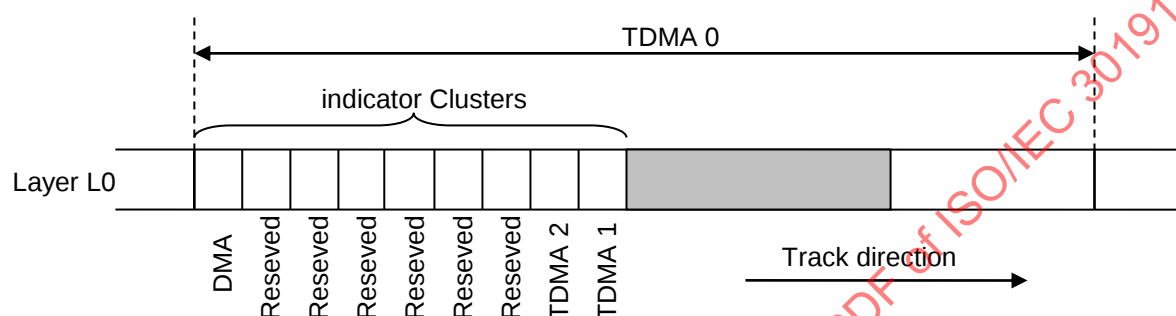
Figure 118 — TDMA Indicator Clusters on TL disk
