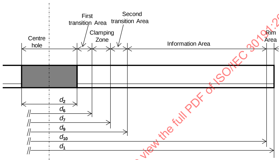
Figure 11 — Overview of disk dimensions
