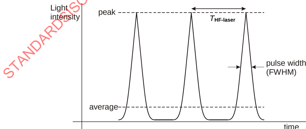
Figure 149 — Schematic representation of light pulses from Laser Diode
