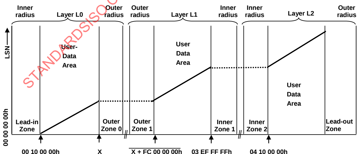
Figure 144 — Assignment of Logical-Sector Numbers
