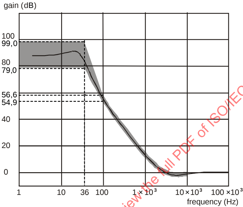
Figure 9 — Servo characteristic for radial tracking at 1x Measurement Velocity
