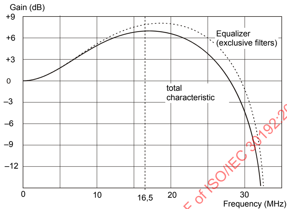
Figure H.1 — Frequency characteristics of Conventional Equalizer
