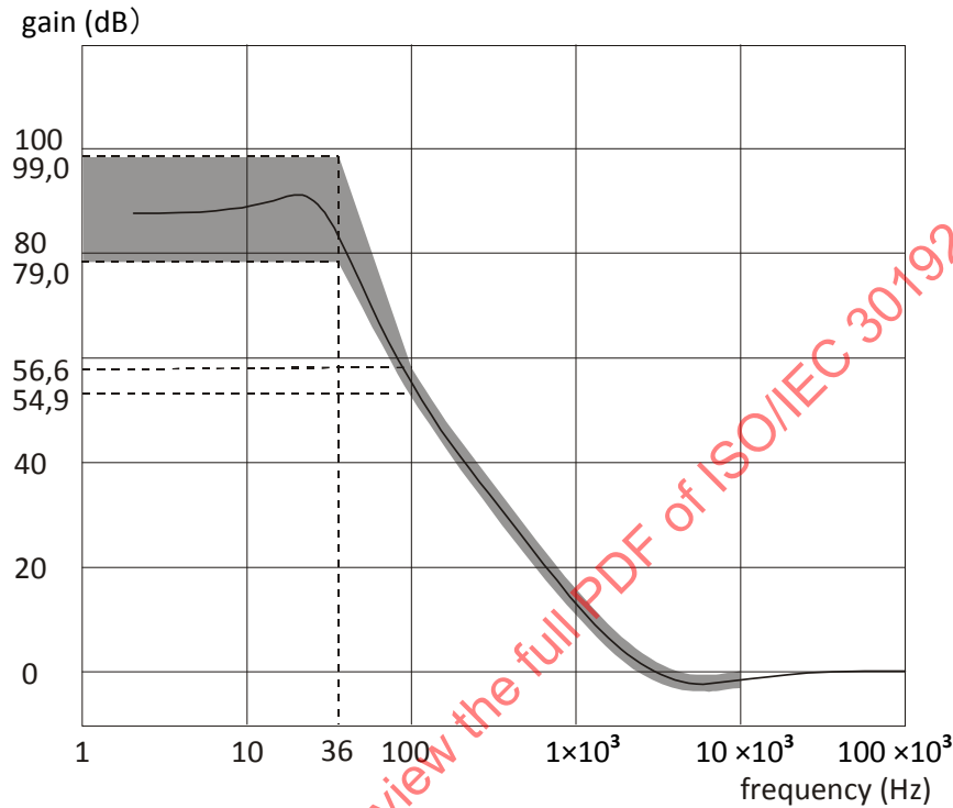
Figure 8 — Servo characteristic for radial tracking
