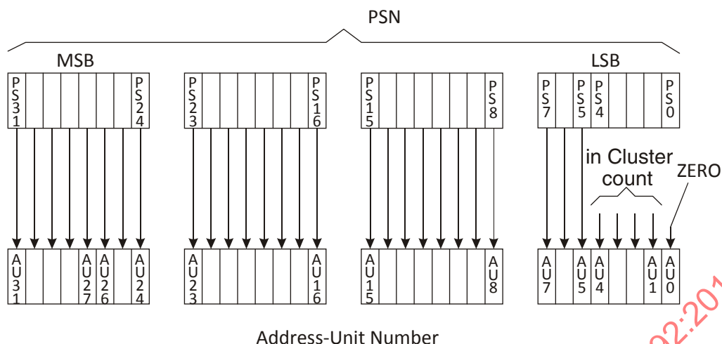
Figure 27 — Composition of AUNs from PSNs
