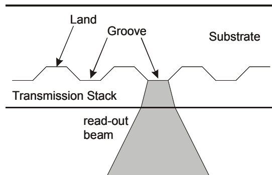
Figure 54 — Outline of Groove geometry (radial cross-section of the disk)
