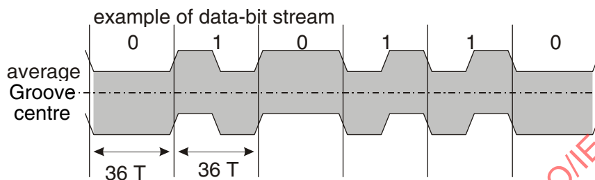
Figure 59 — Biphas modulated HFM Groove
