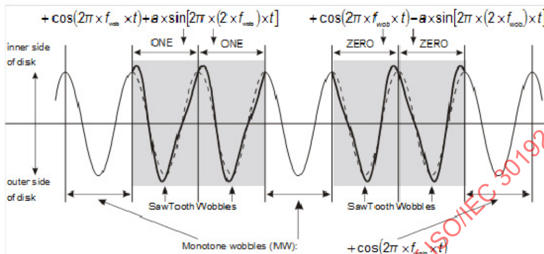
Figure 64 — Definition of Saw-Tooth Wobbles
