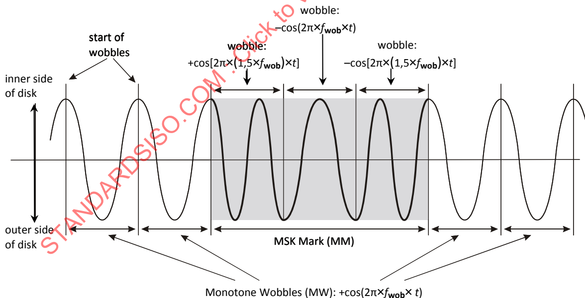
Figure 63 — Definition of MSK Mark
