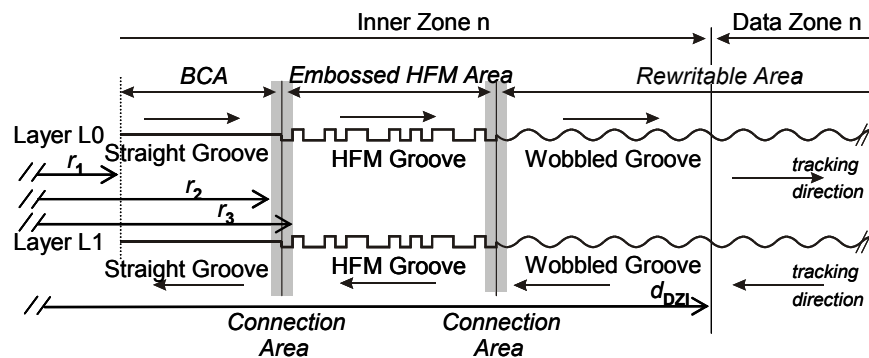
Figure 53 — Connection areas between different Groove types
