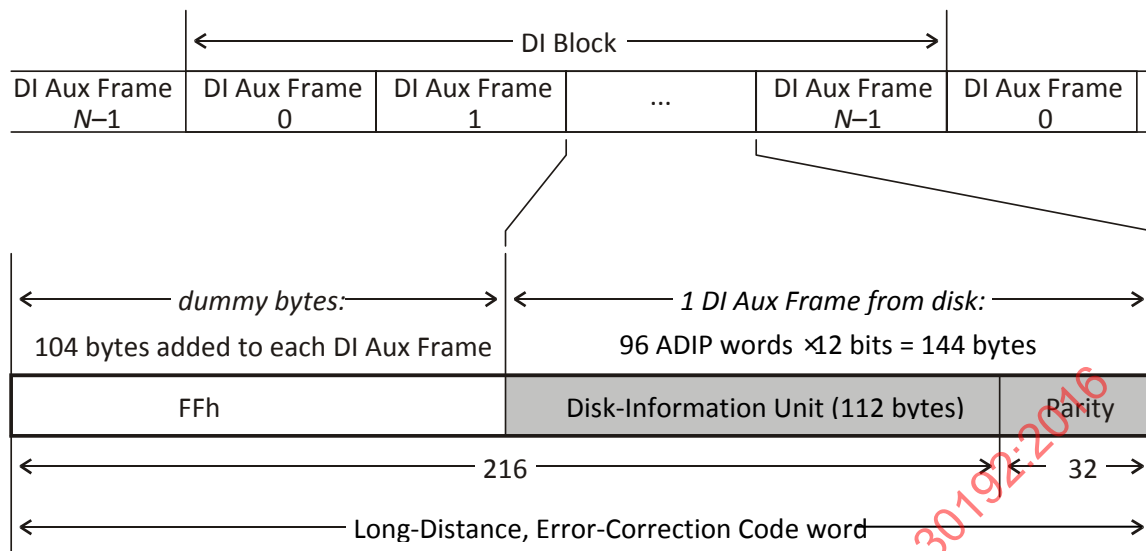
Figure 72 — Disk-Information structure and error-correction format
