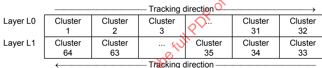
Figure 103 — Clusters of DMA Zones on DL disk
