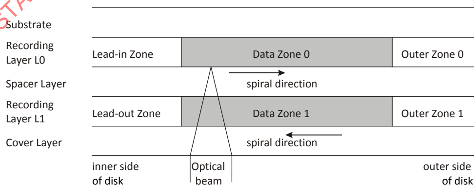
Figure 14 — Subdivision of Information Zone on DL disk
