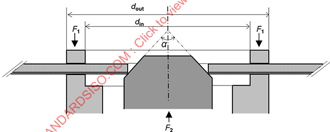
Figure 6 — Clamping conditions for measurement
