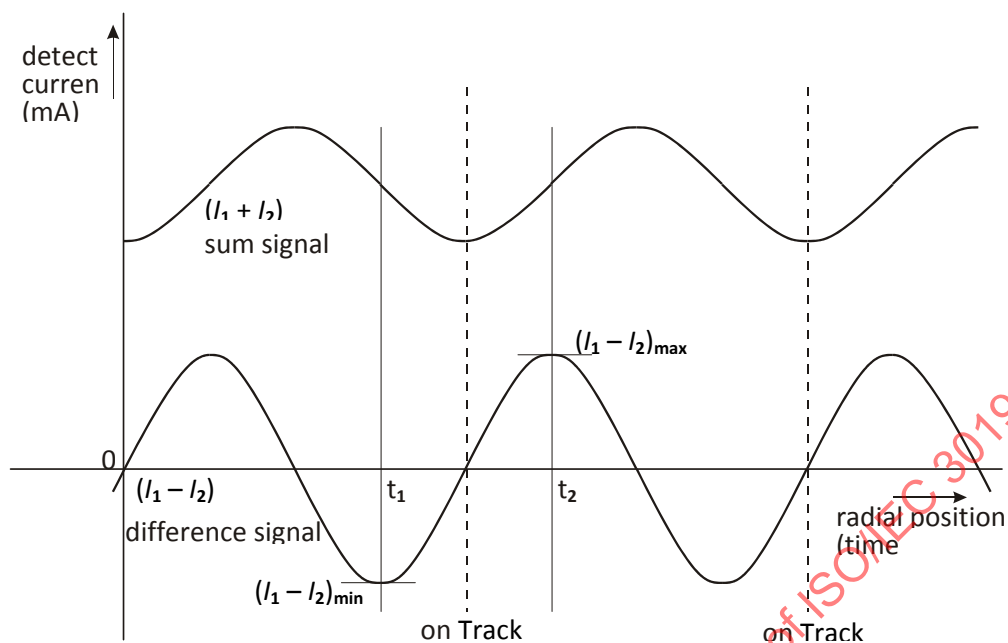
Figure 117 — Definition of Push-Pull signals
