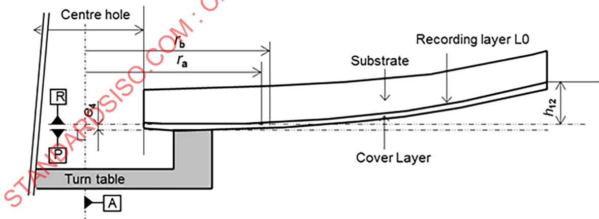
Figure 11 — Details of Disk reference planes P and R and Recording Layer
