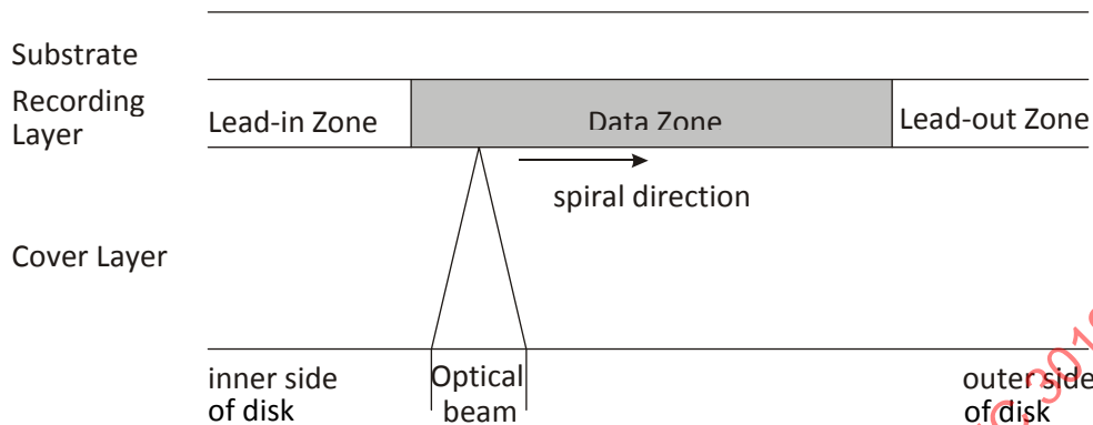
Figure 13 — Subdivision of Information Zone on SL disk
