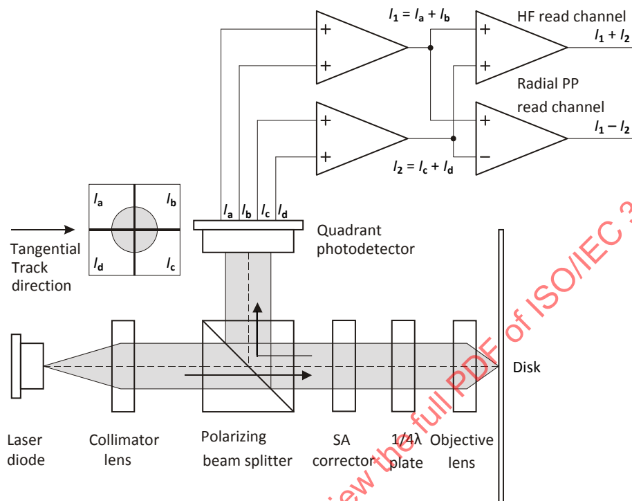
Figure 5 — Optical system of Reference drive
