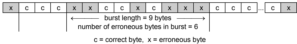
Figure 121 — Example of burst error
