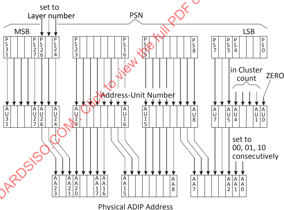
Figure 83 — Physical ADIP Addresses derived from PSNs
