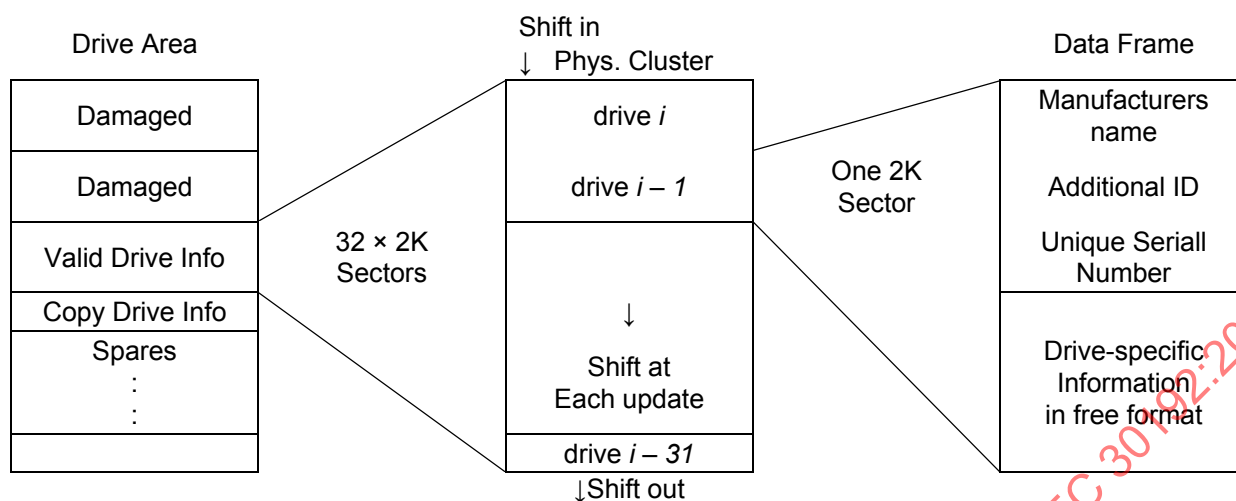
Figure 89 — Format of Drive Area (example)
