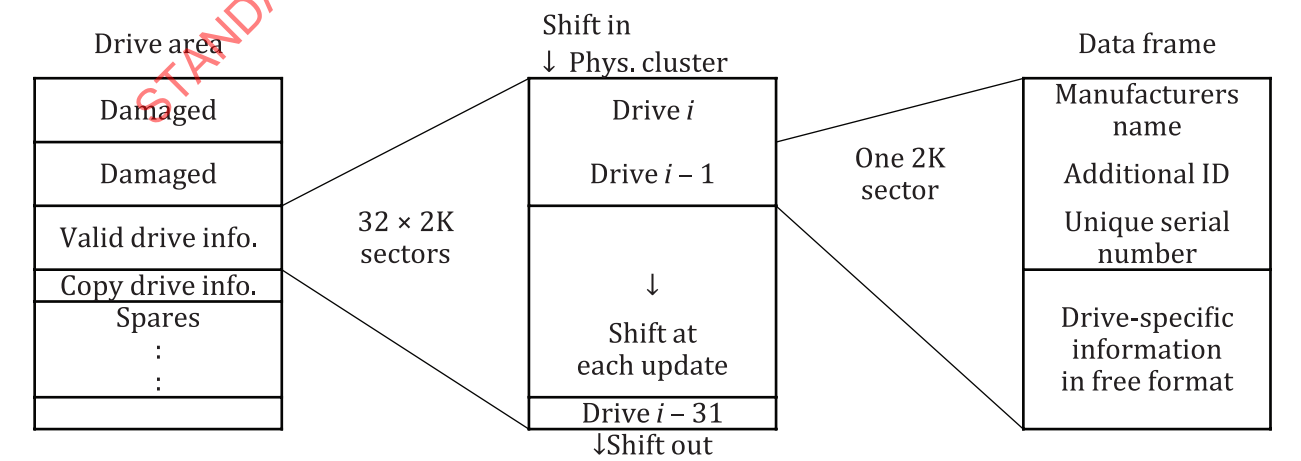
Figure 89 — Format of drive area (example)
