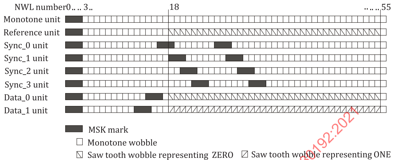
Figure 66 — ADIP unit types
