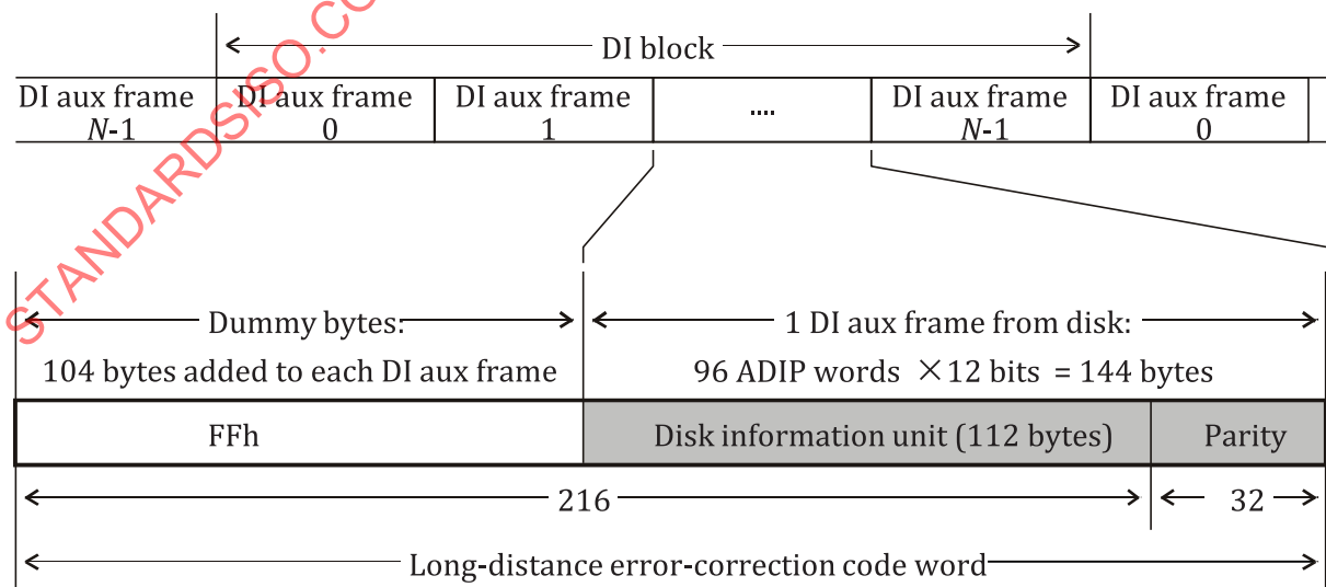
Figure 72 — Disk information structure and error correction format
