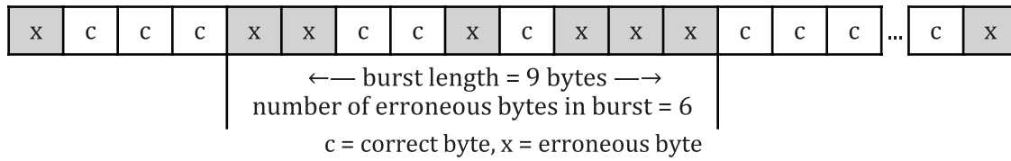
Figure 121 — Example of burst error
