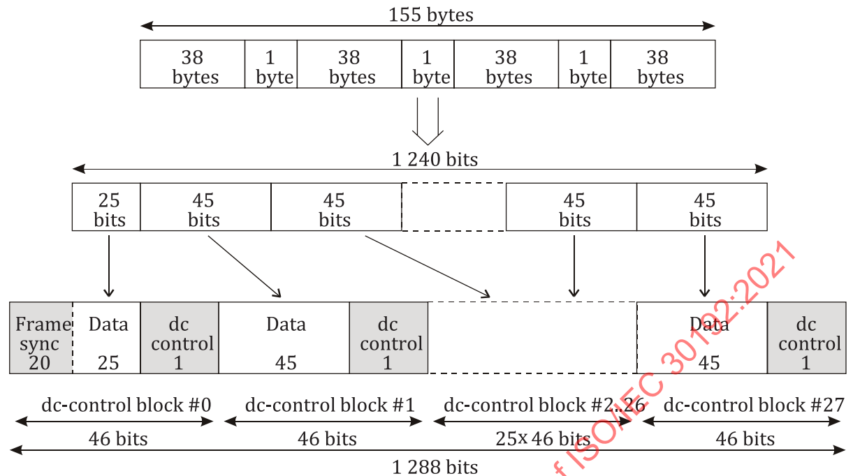
Figure 36 — Composition of recording frame
