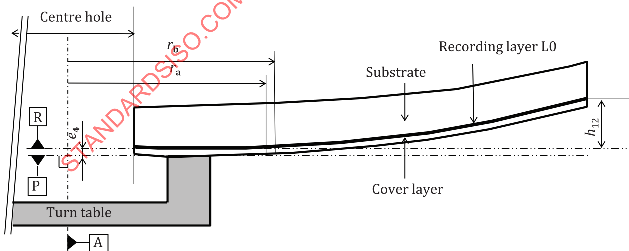
Figure 11 — Details of disk reference planes P and R and recording layer L0
