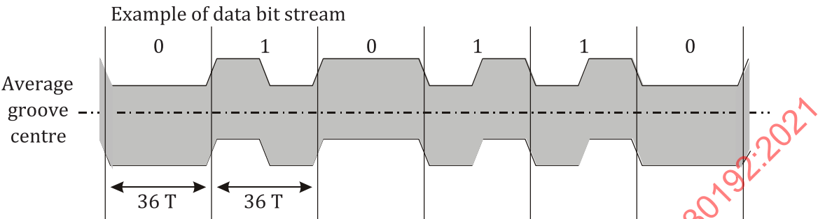
Figure 59 — Biphase modulated HFM groove
