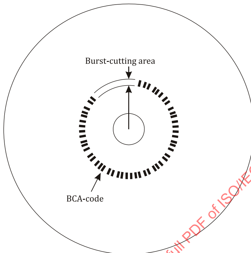
Figure 122 — Schematic representation of BCA
