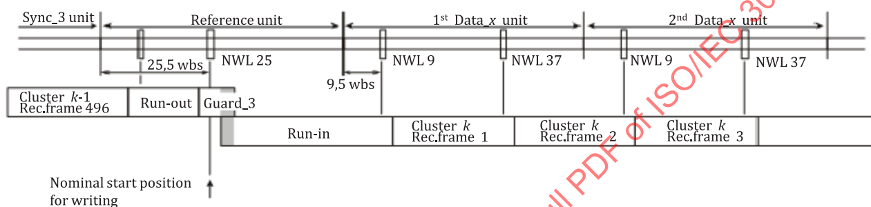
Figure 51 — Example of data recording with maximum overlap
