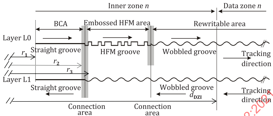
Figure 53 — Connection areas between different groove types
