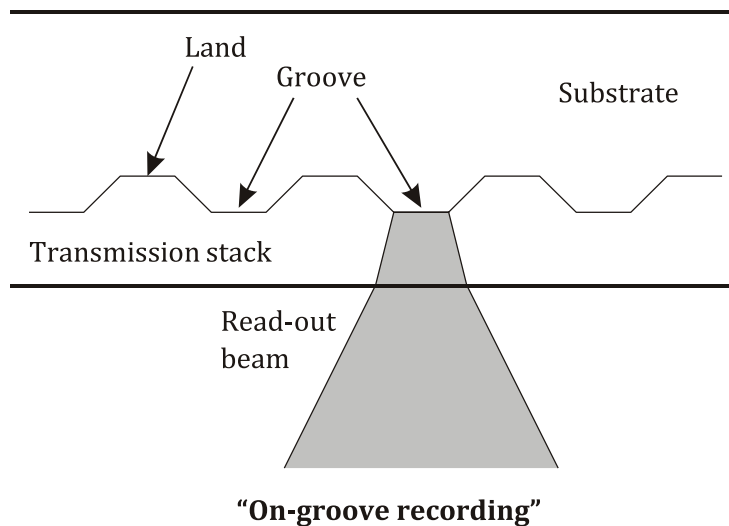
Figure 54 — Outline of groove geometry (radial cross-section of the disk)
