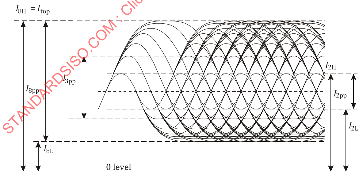
Figure 119 — Schematic representation of HF signal from marks and spaces
