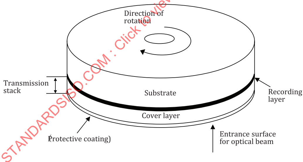
Figure 1 — Outline of type SL disk
