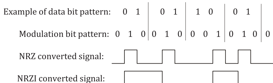
Figure 41 — Modulation and NRZI conversion
