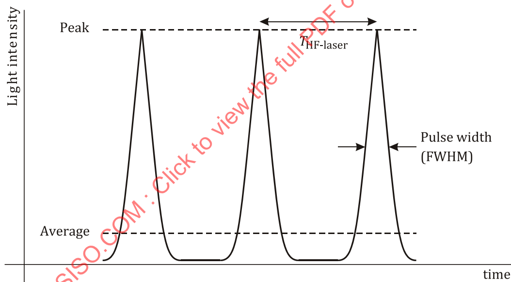
Figure 120 — Schematic representation of light pulses from laser diode
