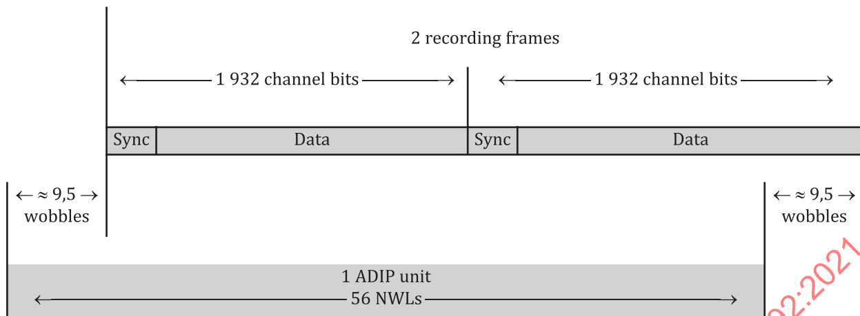
Figure 65 — General ADIP structure
