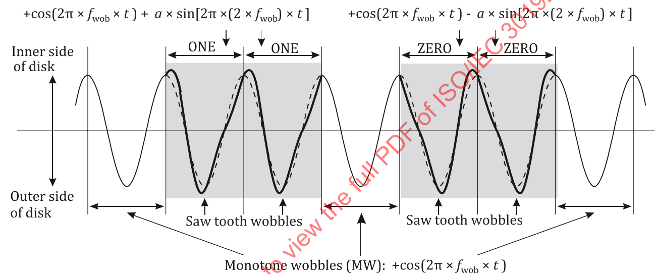
Figure 64 — Definition of saw-tooth wobbles
