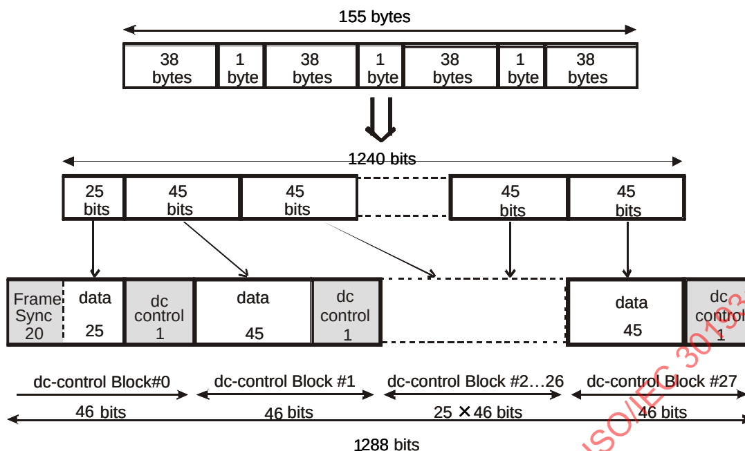
Figure 35 —Composition of Recording Frame
