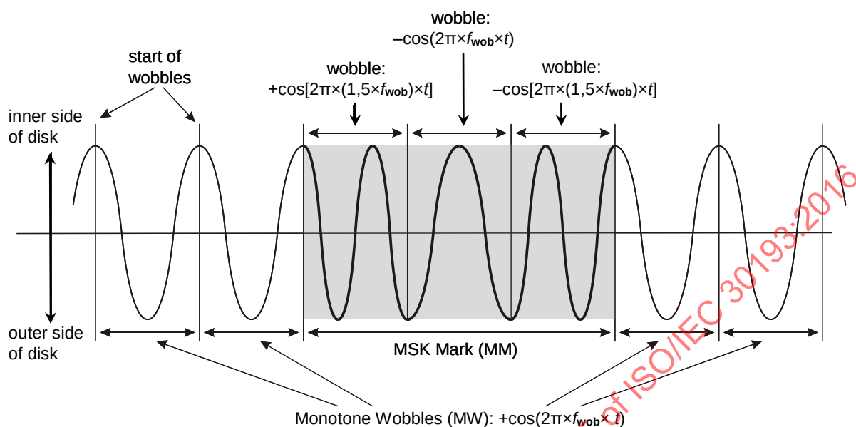
Figure 62 — Definition of MSK Mark (on-Groove)
