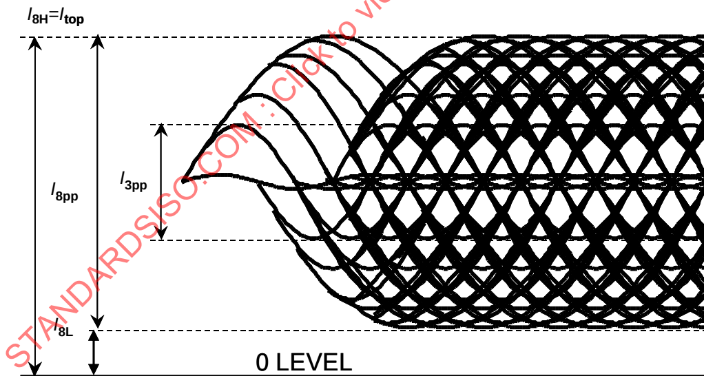
Figure 119 — Schematic representation of HF signal from Marks and Spaces
