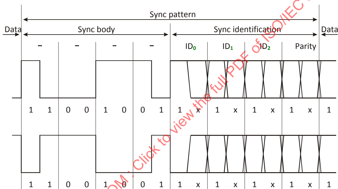
Figure 59 — Biphase Synchronization pattern
