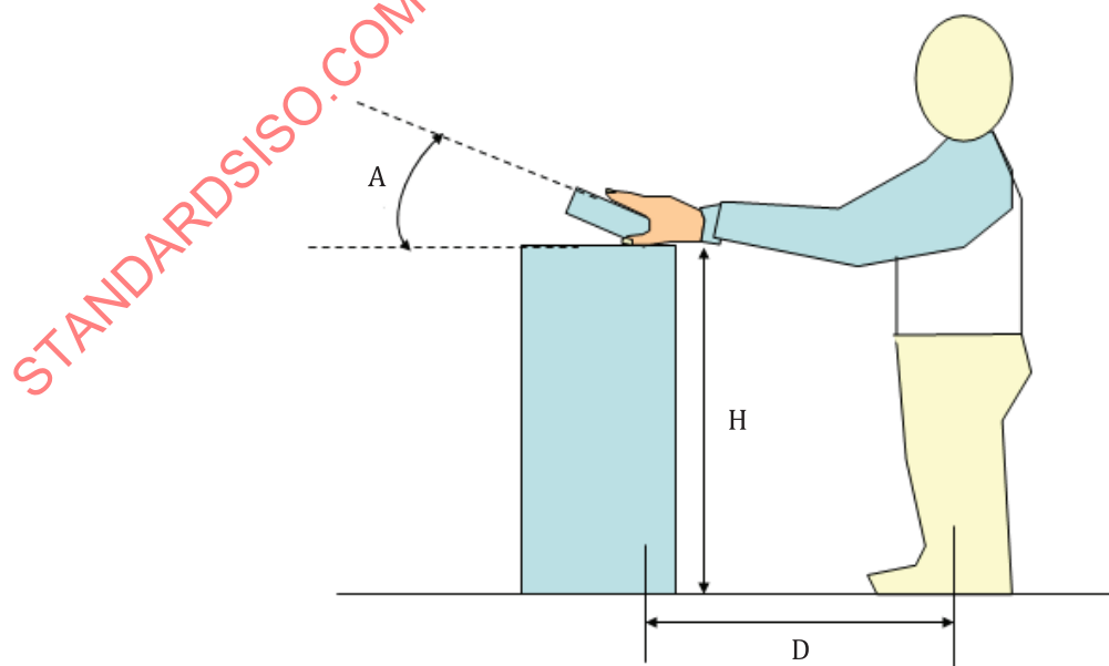
Figure E.7 — Standing position
