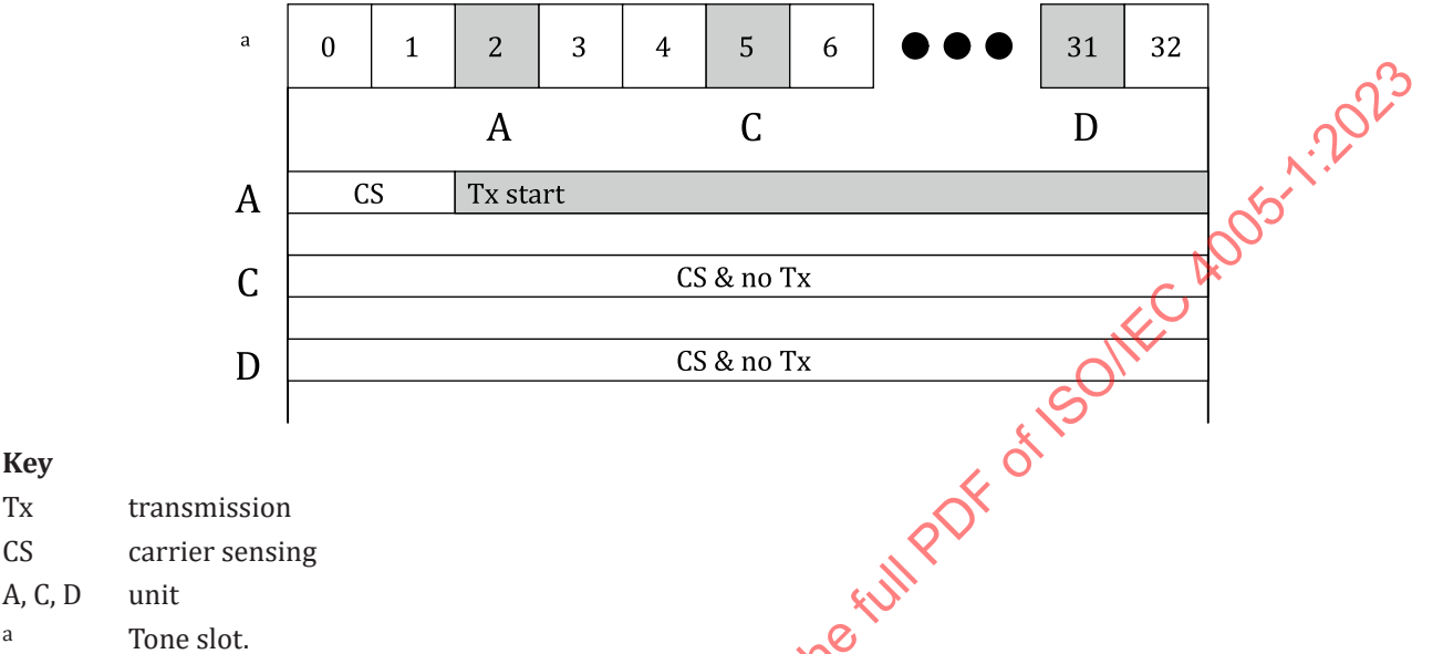
Figure 6 — First competition example
