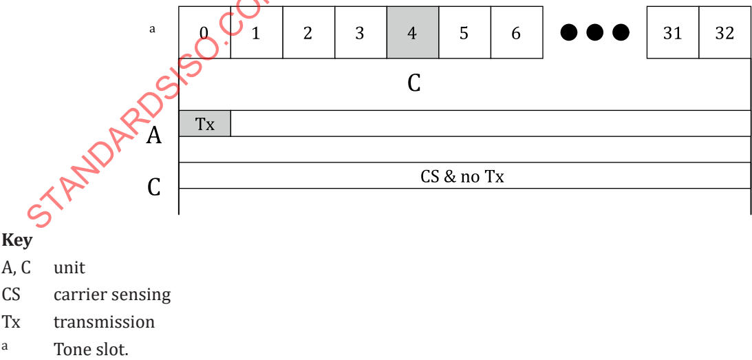
Figure 8 — Slot clearing example
