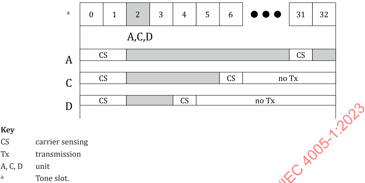
Figure 7 — Second competition example
