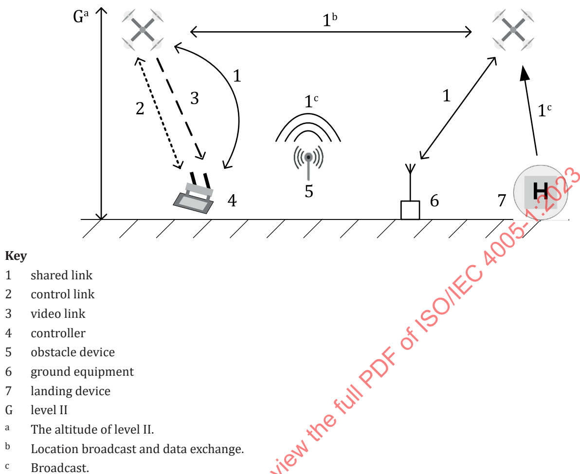
Figure 1 — Three types of communications
