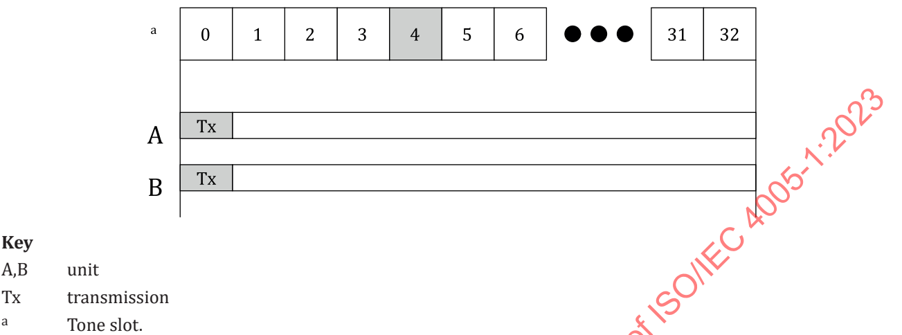
Figure 9 — Slot clearing example for hidden node removal
