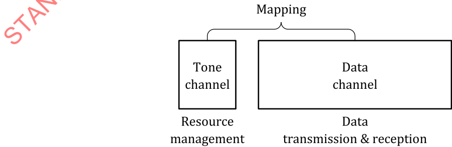
Figure 2 — Multichannel structure and the role of each channel
