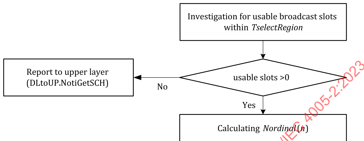
Figure 13 — Selection procedure for a broadcast slot to attempt allocation
