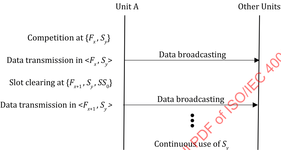
Figure 16 — Procedure for allocation and occupation of broadcast slot
