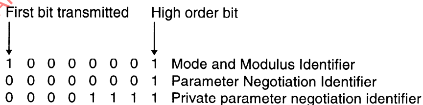
Figure 15 — Data link layer subfield encodings
