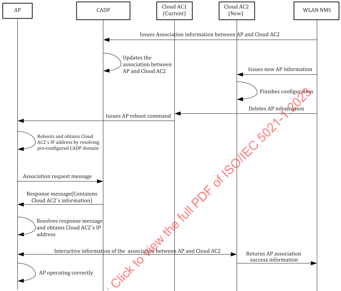
Figure 4— Cloud AC switchover for optimization or replacement
