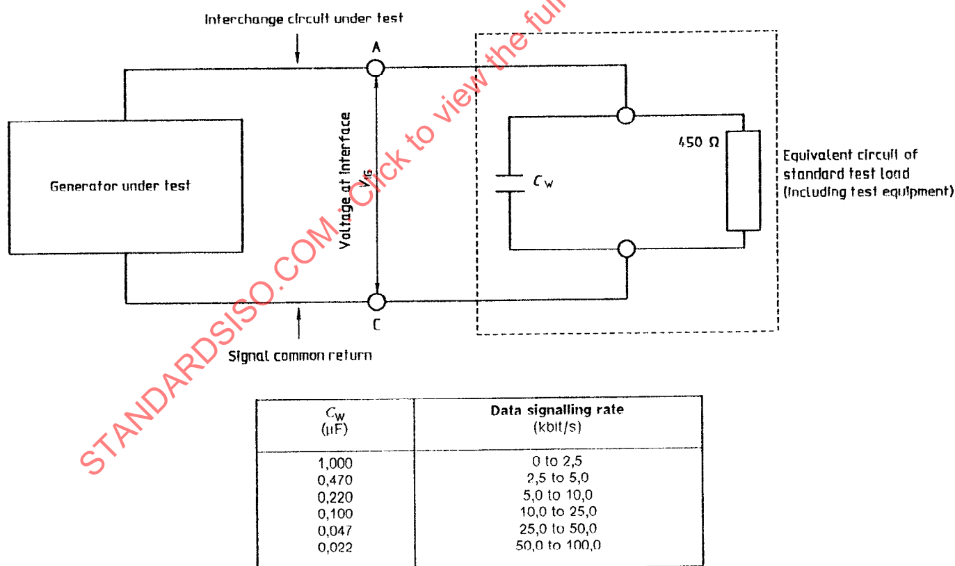
Figure 3 — Test arrangement for V.10 generators and values of C_w
