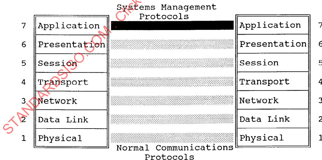
Figure A.1 - Systems Management Information Exchange
