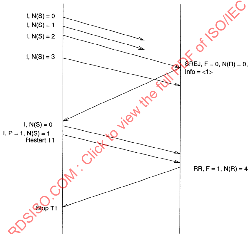
Figure C-1: I frame recovery due to SREJ frame with F bit set to "0"
