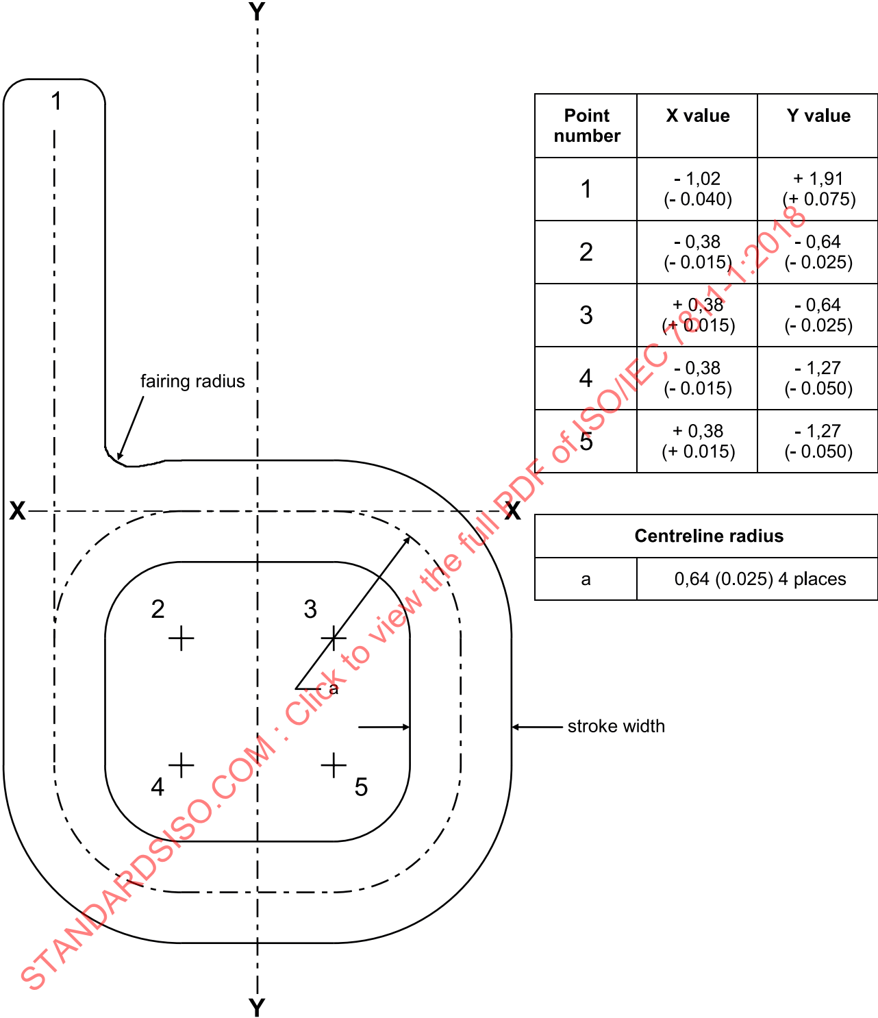
Figure B.6 — Printed image for 7B font-6
