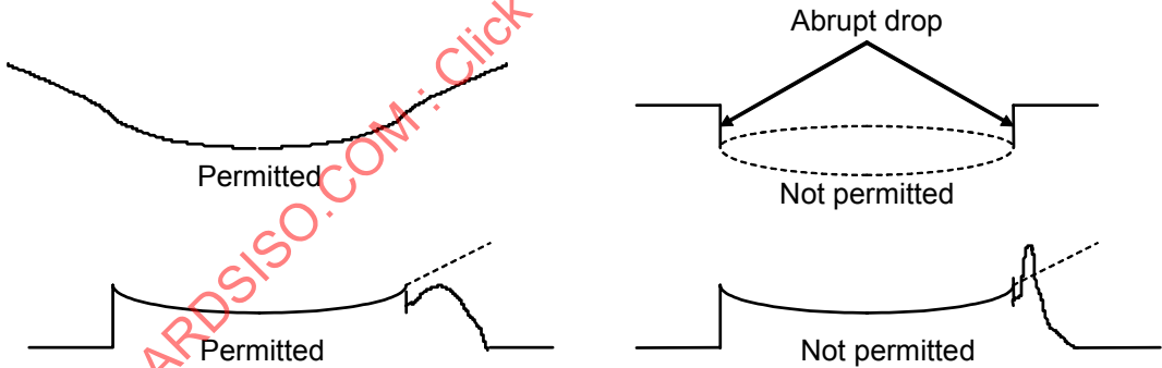
Figure 4 — Surface profile examples
