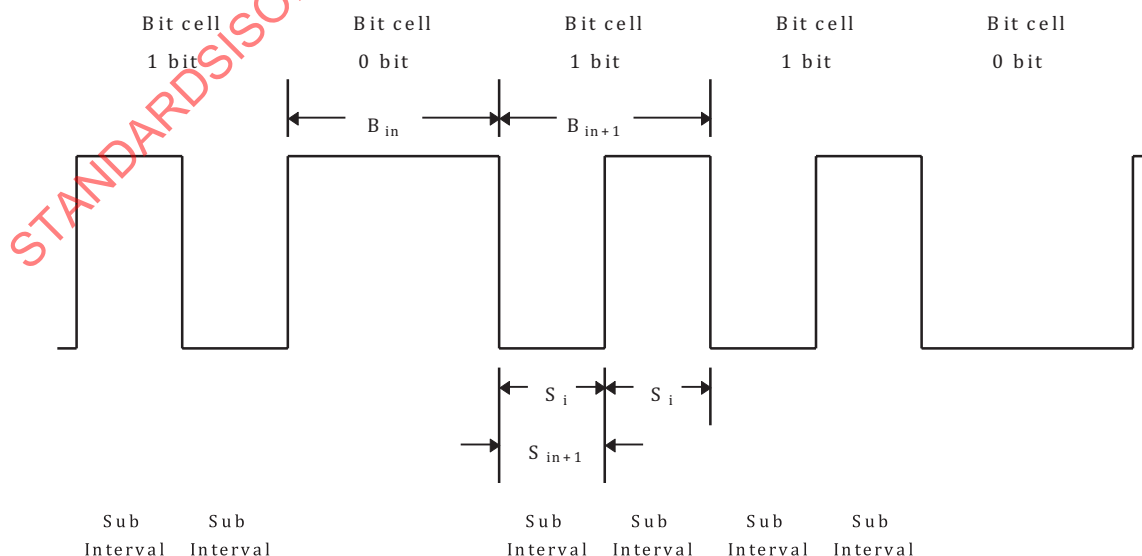
Figure 11 — Flux transition spacing variation
