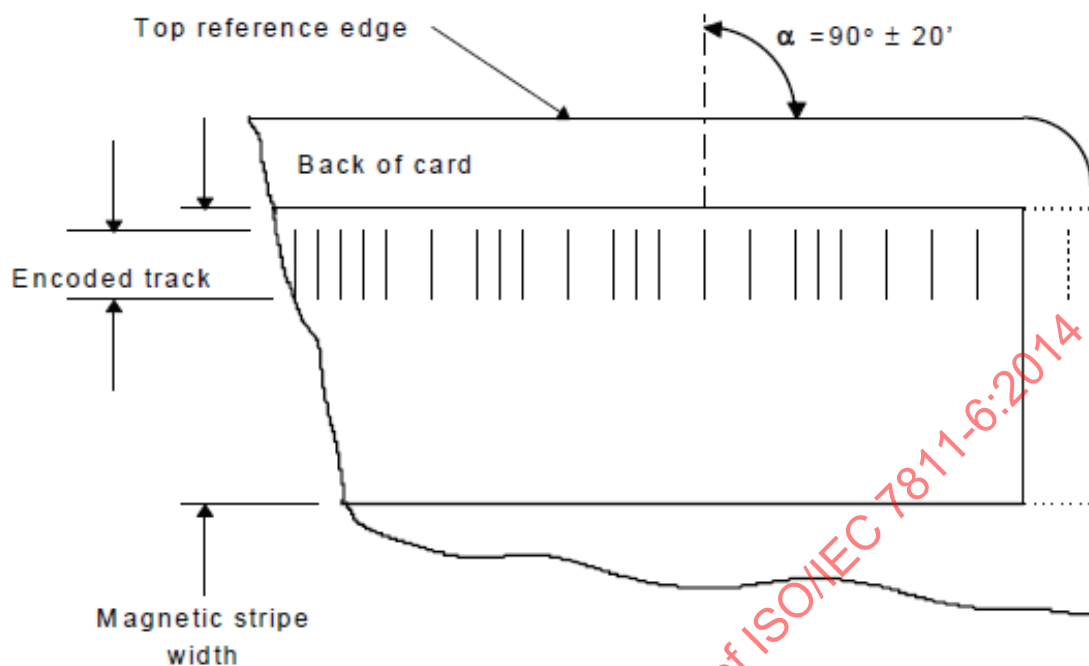
Figure 9 — Angle of recording
