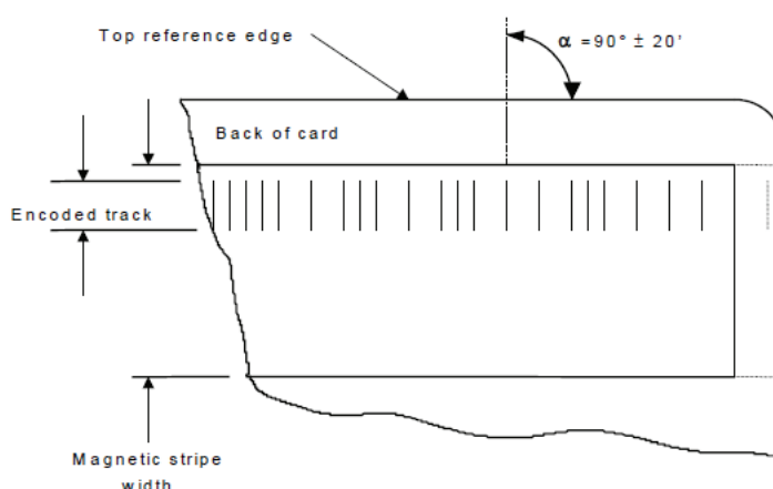
Figure 9 — Angle of recording
