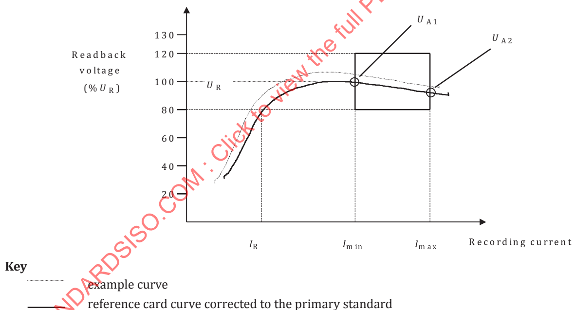
Figure 6 — Saturation curve example showing tolerance area
