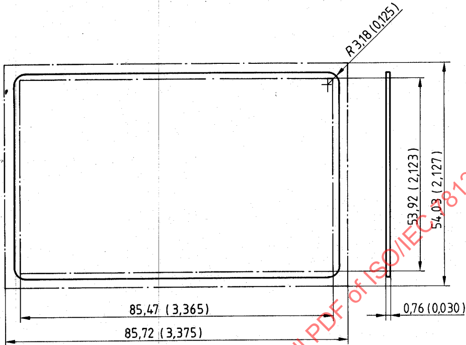
Figure 1 — Card dimensions
