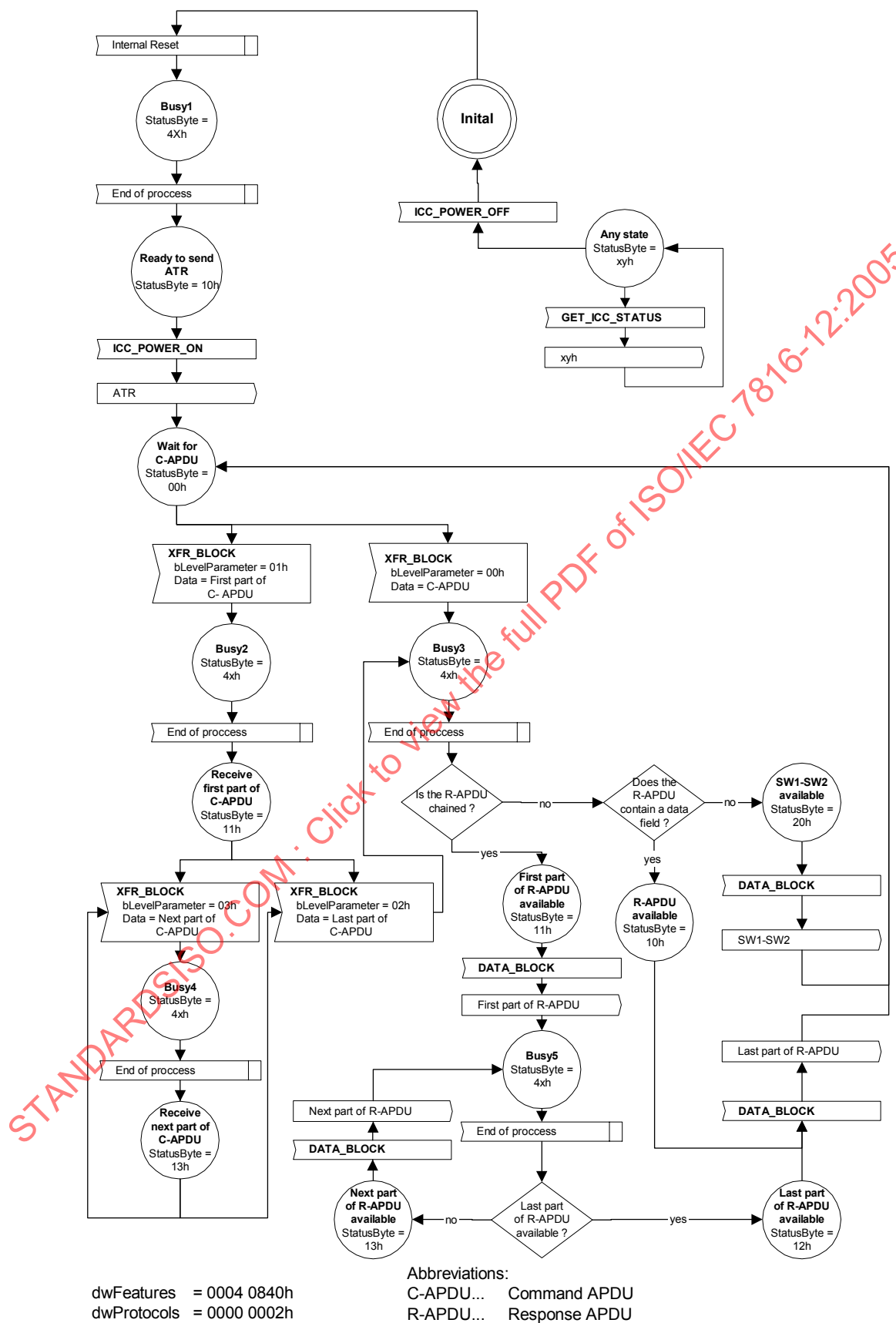
Figure 5 — State diagram of the USB-ICC for control transfer (Version A) using extended APDUs
