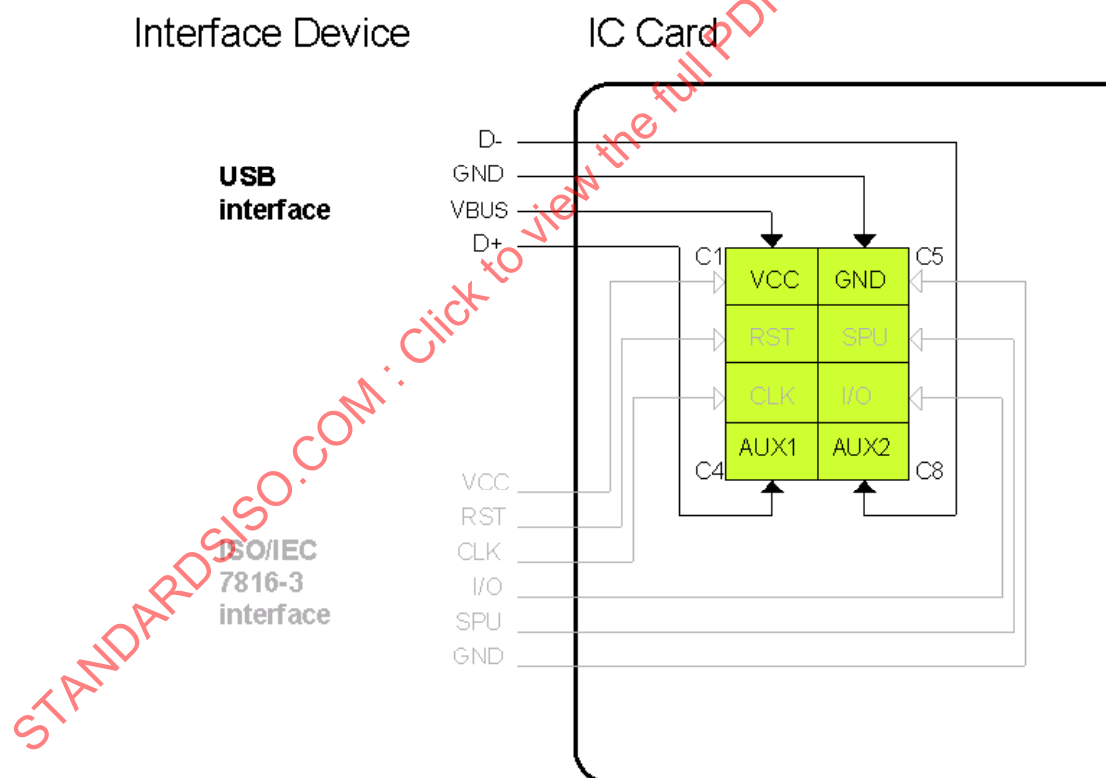
Figure 1 — Assignment of contacts for a USB integrated circuit card
