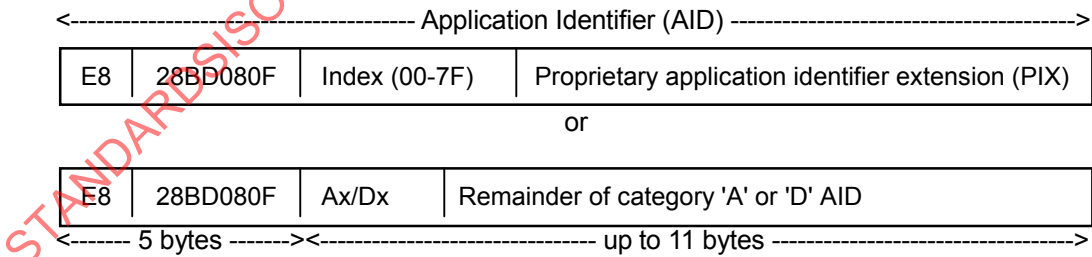
Figure 6 — AID formats
