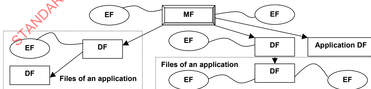
Figure 3 — Example of hierarchy of DFs
