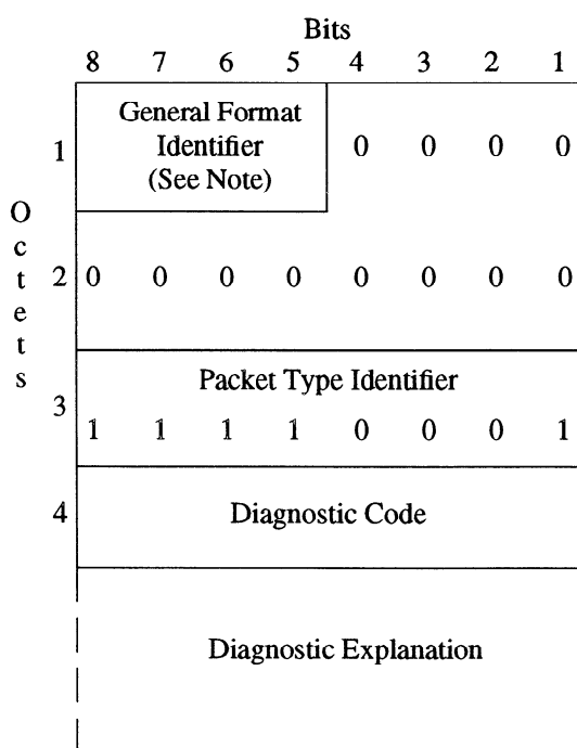
Figure 26 — DIAGNOSTIC Packet Format
