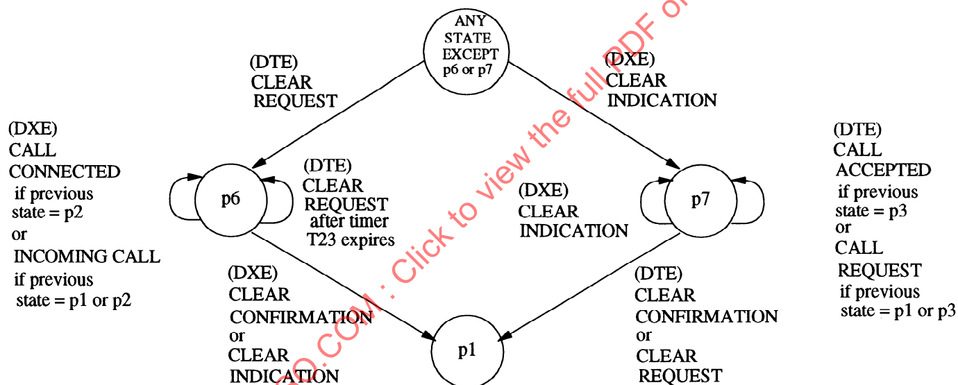
(b) CALL CLEARING PHASE
