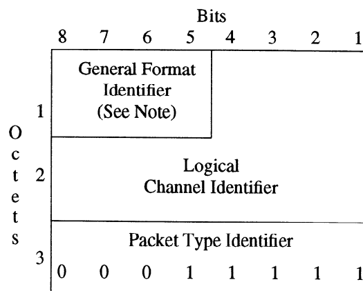
Figure 23 — RESET CONFIRMATION Packet
