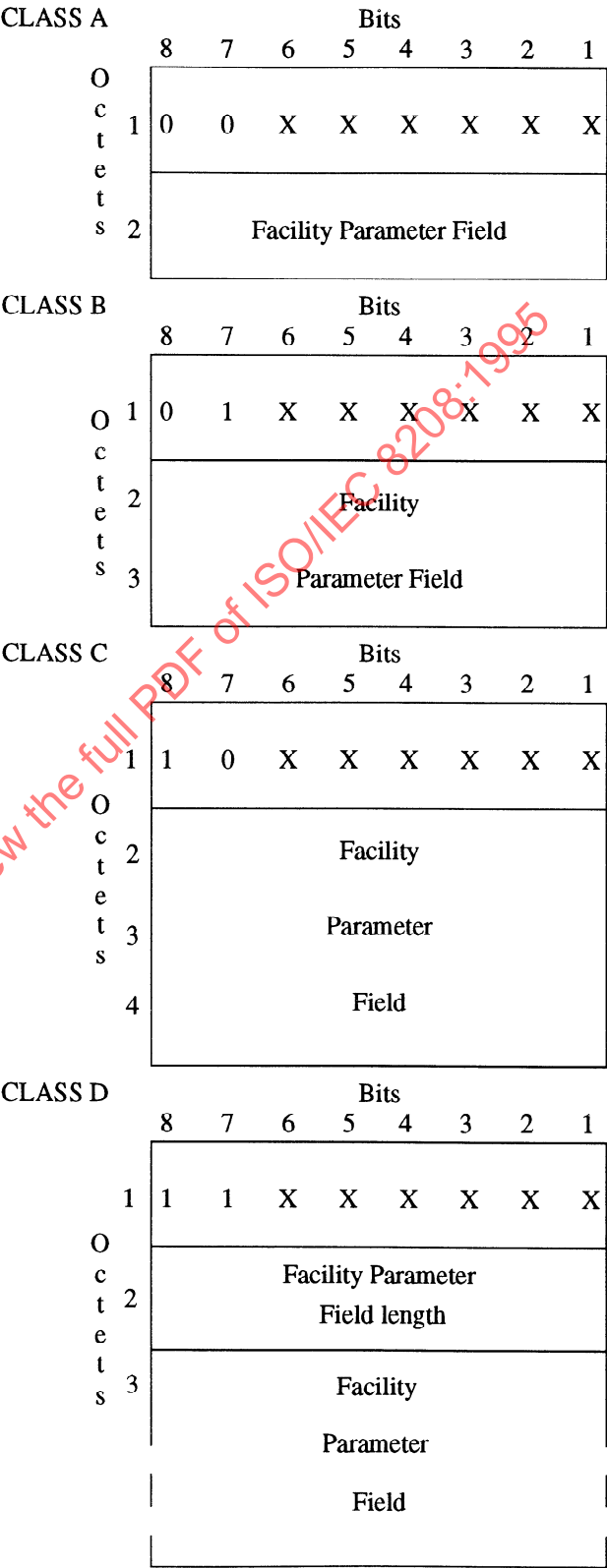
Figure 32 — Generalized Formats of Facility Elements
