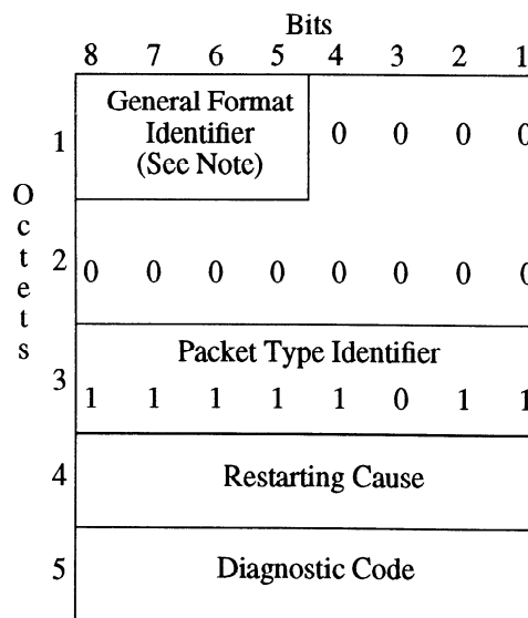
Figure 24 — RESTART REQUEST and RESTART INDICATION Packet Format
