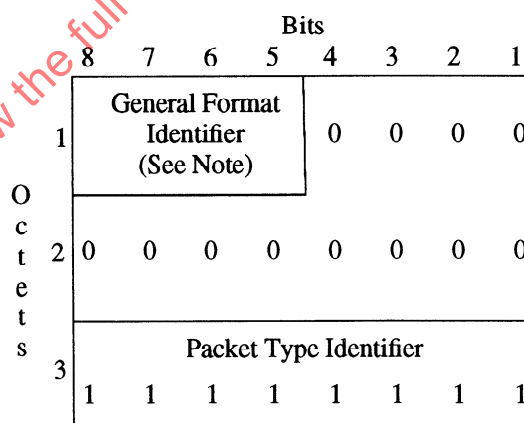
Figure 25 — RESTART CONFIRMATION Packet Format
