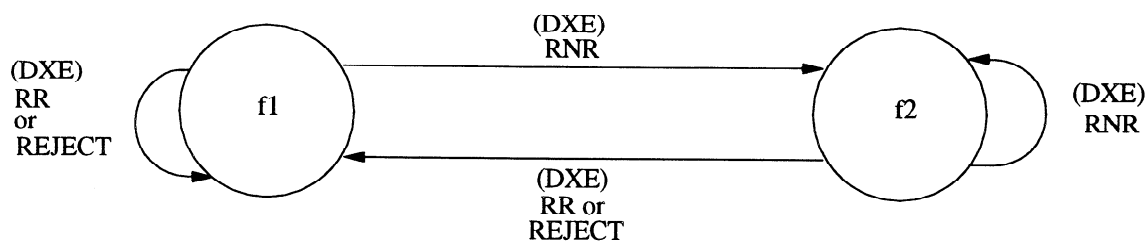
(a) FLOW CONTROL FROM DXE TO DTE (DATA TRANSFER FROM DTE TO DXE)
