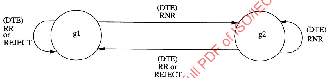
(b) FLOW CONTROL FROM DTE TO DXE (DATA TRANSFER FROM DXE TO DTE)
