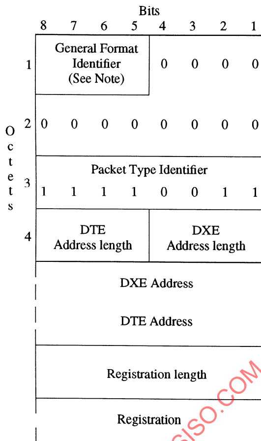
Figure 28 — REGISTRATION REQUEST Packet Format
