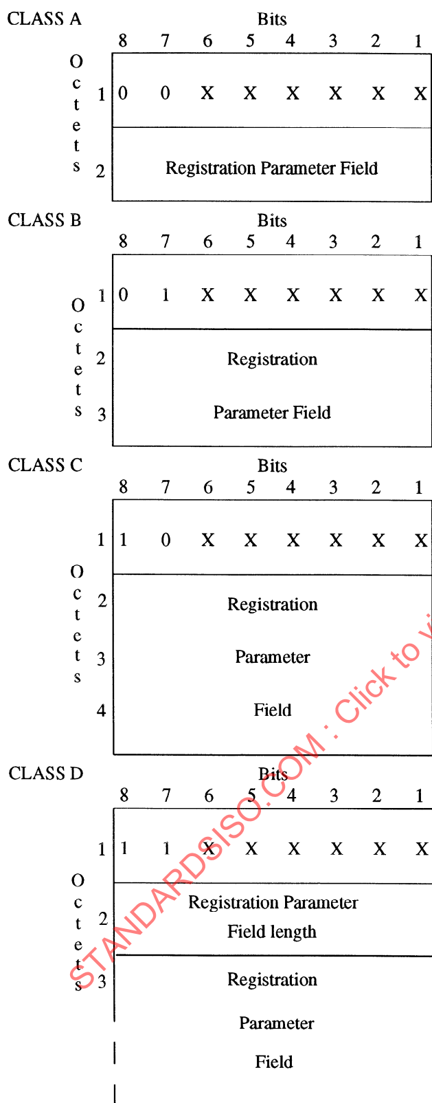
Figure 33 — Generalized Formats of Registration Elements
