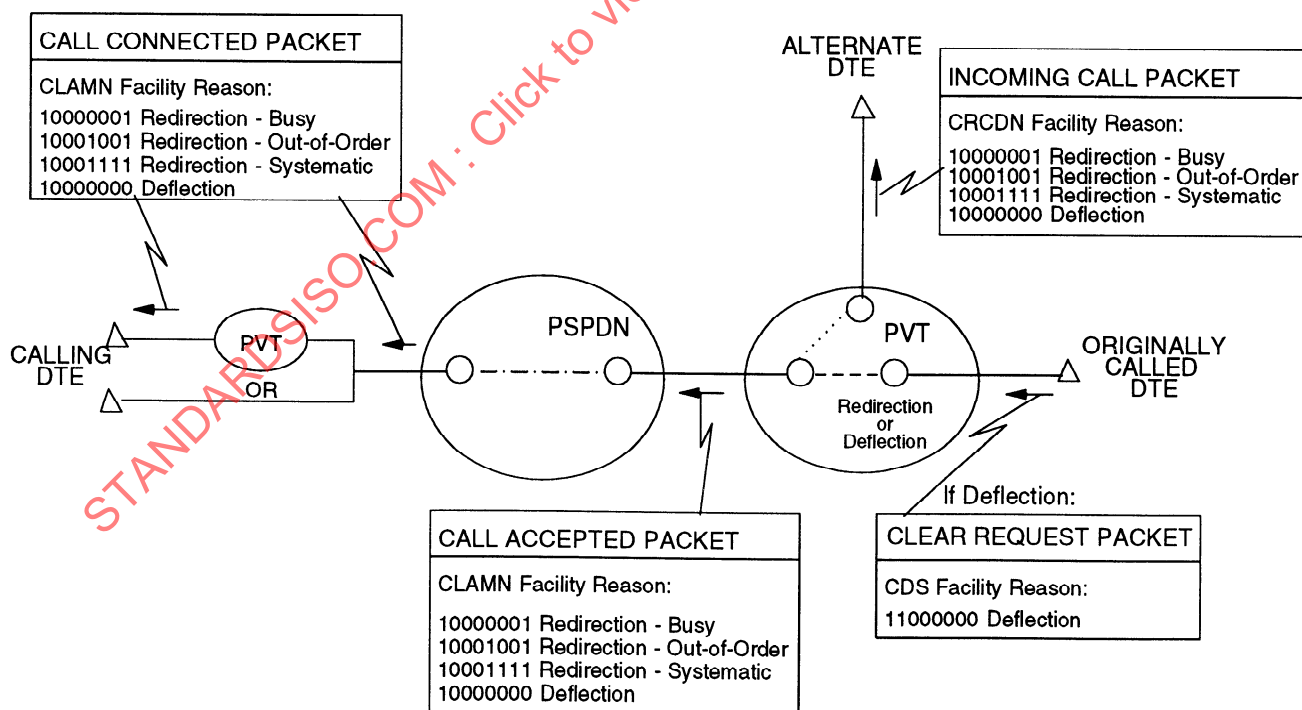
Figure A.2 (2 of 3) — Call Redirection and Call Deflection operation
