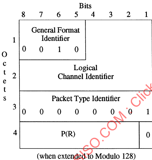
Figure 20 — RECEIVE READY Packet Format
