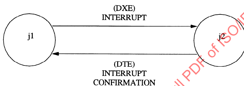
(b) INTERRUPT TRANSFER FROM DXE TO DTE
