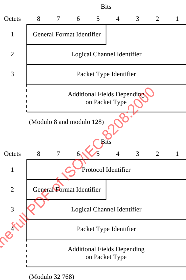
Figure 10 — General Packet Format
