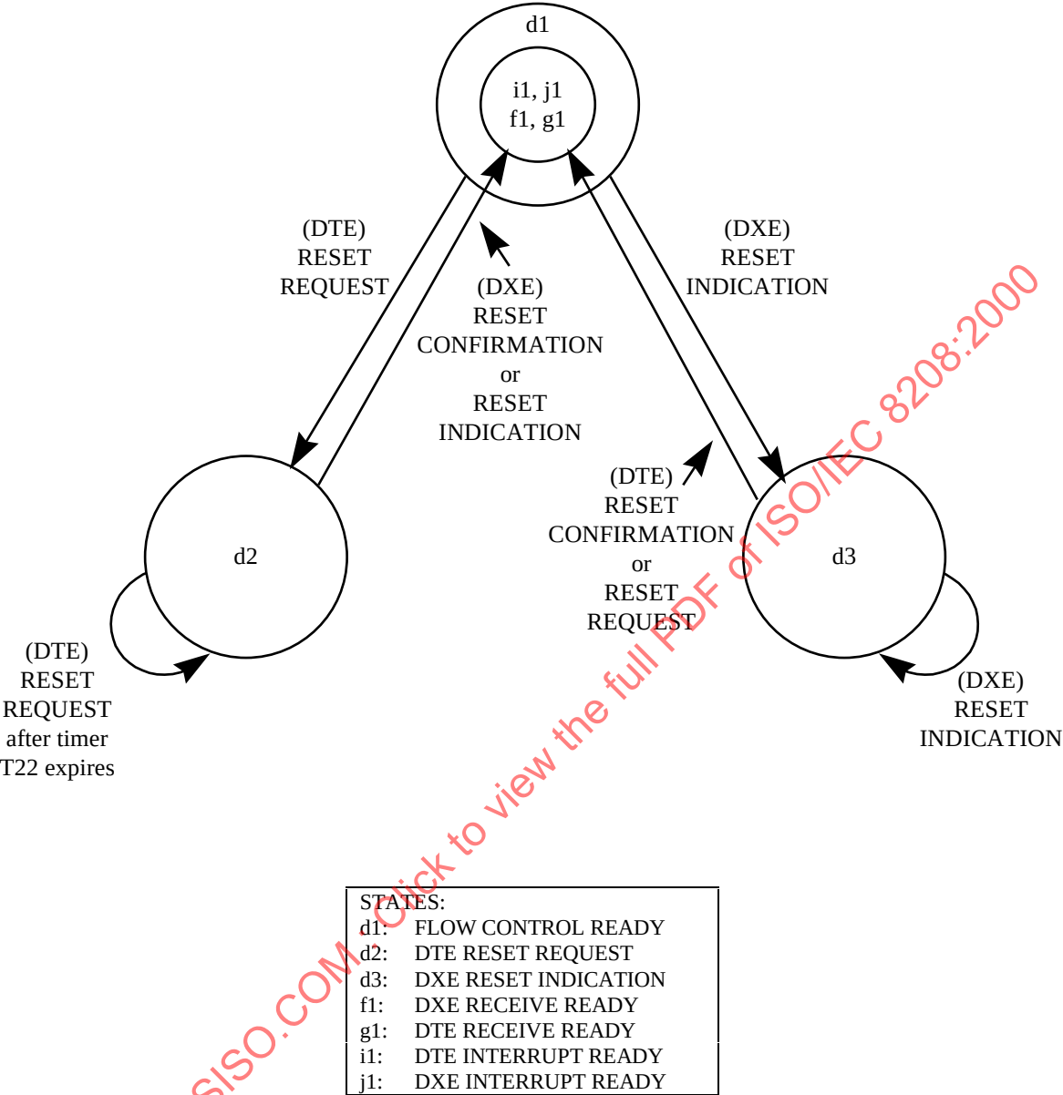
Figure 36 — State Diagram for the Transfer of Reset Packets within the Data Transfer State (p4)
