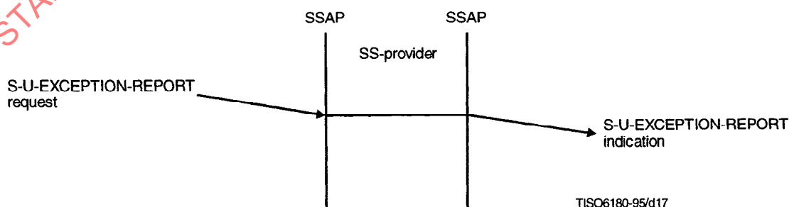
Figure 16 – U-exception report time sequence diagram
