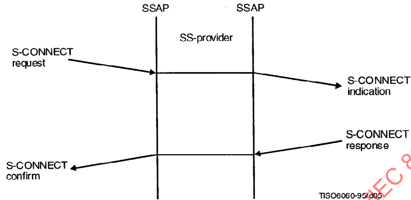
Figure 4 – Scssion connection establishment time sequence diagram
