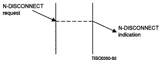
Figure 6 – Sequence of primitives in NS user invoked NC release
