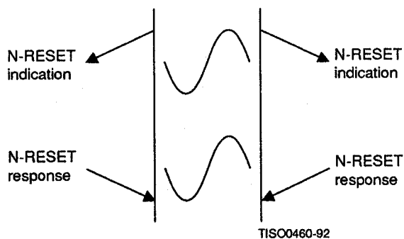
Figure 17 – Sequence of primitives in NS provider invoked reset
