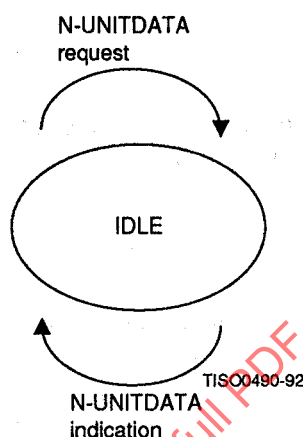
Figure 20 – State transition diagram for sequences of connectionless-mode primitives at one NSAP
