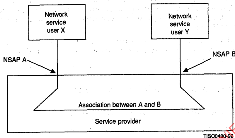
Figure 19 – Model of a network-connectionless-mode-transmission
